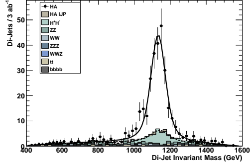
Figure 3. b\bar{b} invariant mass distribution showing the e^+e^- \rightarrow H^0A^0 \rightarrow b\bar{b}b\bar{b} signal above the SM and SUSY backgrounds for M_A = 1.14 \text{ TeV} at \sqrt{s} = 3 \text{ TeV} and assuming a b -tagging efficiency \epsilon_b = 0.85 . The result is obtained with full simulation and reconstruction of a detector at CLIC (from [12]).
