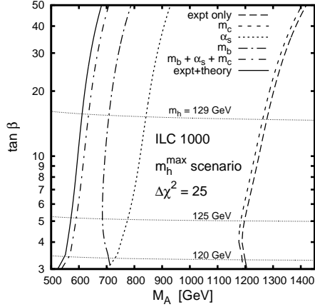
Figure 2. Contributions of different sources of parametric uncertainties to the sensitivity to M_A from measurements of the h^0 couplings in SUSY (from [11]).
