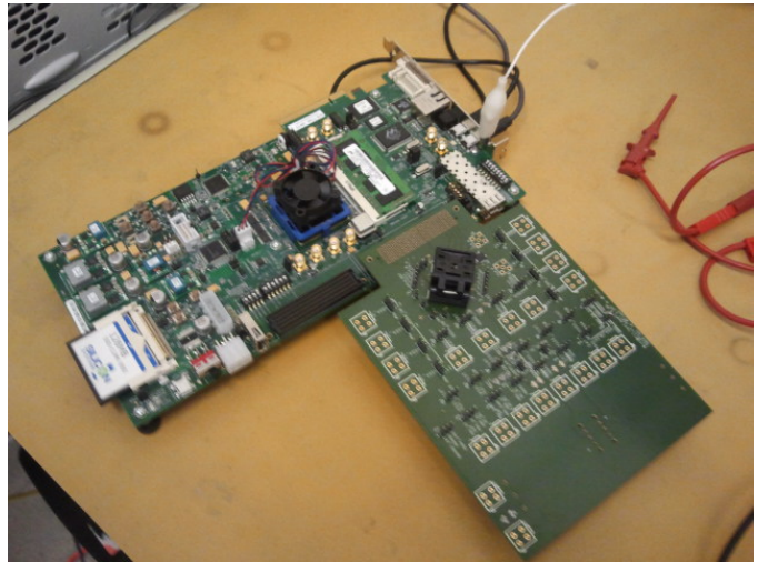
Fig. 5. AMchip mini@sic test setup
