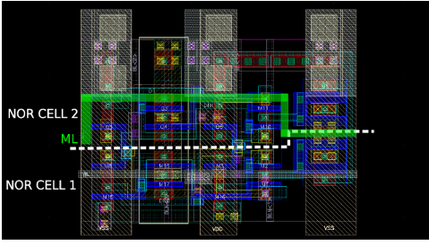
Fig. 3. AMchip05 CAM NOR cell layout
