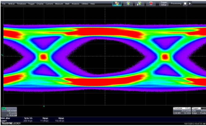
Fig. 6. AMchip mini@sic SER eye diagram at 2 Gbps
