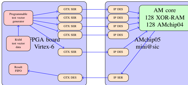
Fig. 7. AMchip mini@sic test setup scheme
