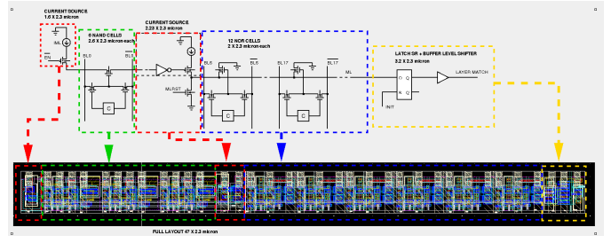
Fig. 4. AMchip05 CAM cell scheme
