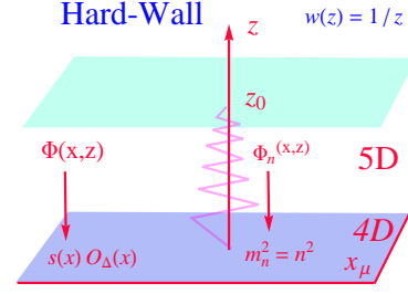
Figure 1. A pictorial representation of a Hard-Wall model. The 5D metric is AdS 5 with warp factor w(z) = 1/z . The extradimension z is sharply cut-off at a value z_0 . This compactification generates an infinite series of 5D normalizable modes \Phi_n(x, z) corresponding to an infinite tower of 4D resonances with masses m_n^2 \propto n^2 . The mass scale is fixed by the value of the dimensional parameter z_0 .
