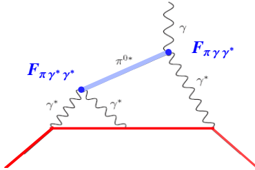
Figure 3. The neutral pion exchange diagram in the hadronic light-by-light scattering contribution to (g-2)_\mu
