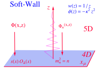
Figure 2. A pictorial representation of the Soft-Wall model. The 5D metric is AdS 5 with warp factor w(z) = 1/z and with unbounded extradimension z . In presence of the dilaton background \phi(z) = -\kappa^2 z^2 , an infinite series of 5D normalizable modes \Phi_n(x, z) is produced, and hence 4D resonances with masses, m_n^2 \propto n , following a Regge behavior. The mass scale is fixed by the value of the dimensional parameter \kappa .
