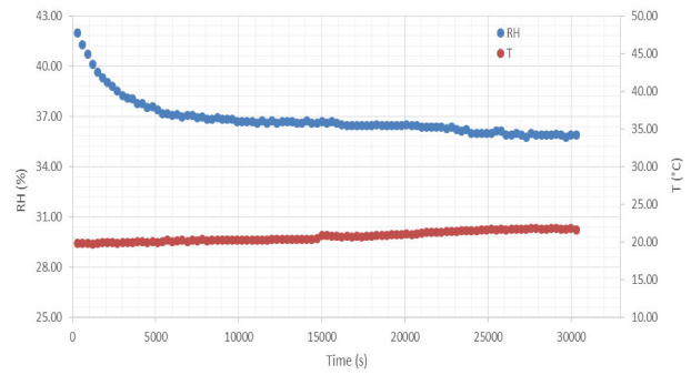
Figure 7. Temperature and relative humidity vs. time within the glass vessel during the test.
