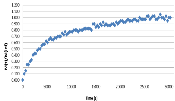
Figure 8. Humidity saturation trends in the GEM foil sample.
