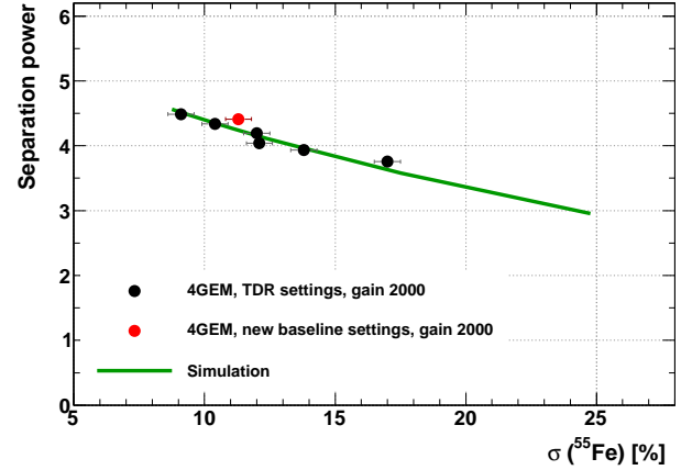
Figure 5. Separation power of pions and electrons with a momentum of 1 GeV/c as a function of the ^{55}\text{Fe} resolution at a gain of 2000. The green curve shows the result of a simulation. Reproduced from [5].
