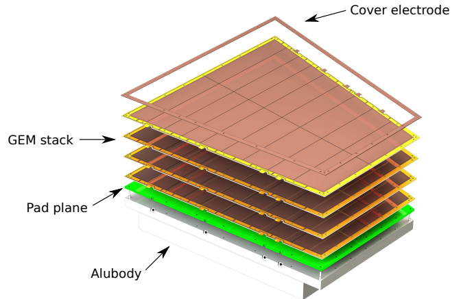
Figure 2. Exploded view of the IROC prototype with the individual components being depicted.
