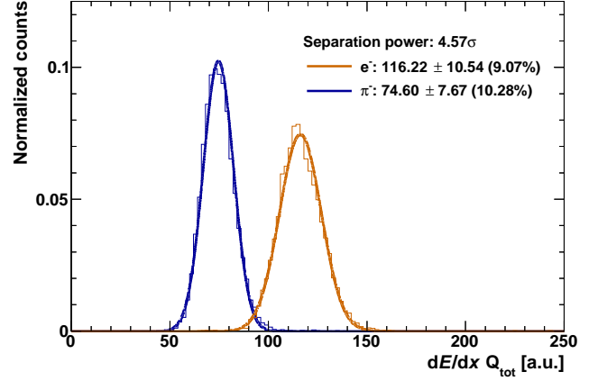
Figure 4. Truncated (0–70%) energy loss distributions for electrons (orange) and pions (blue) with 1 GeV/c momentum measured with the IROC GEM prototype at a gain of 2000.
