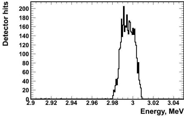
Figure 3. Spectrum of electrons at the exit of LEETECH facility.
