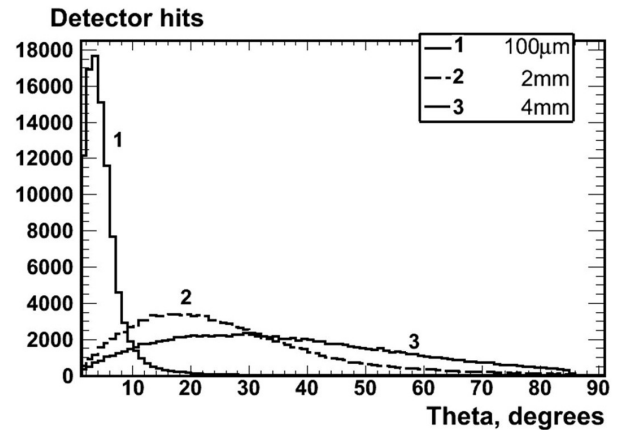
Figure 6. Angular distribution of electrons' direction after the attenuator.
