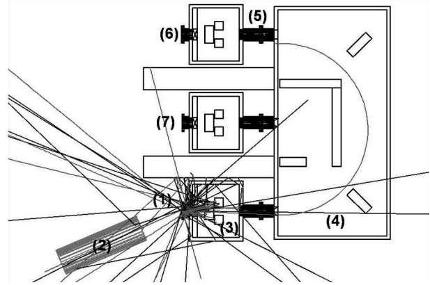
Figure 2. Geometry implemented into full Geant4 simulation. End of the PHIL beam pipe (2), target (1), vacuum chamber with magnetic field (4), entrance and exit collimator systems (3, 5) and lead shielding are shown.
