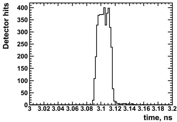
Figure 4. LEETECH timing characteristics for "narrow" mode of collimator system.
