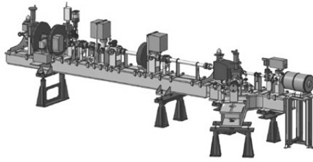
Figure 1. General view of PHIL photoinjector.
