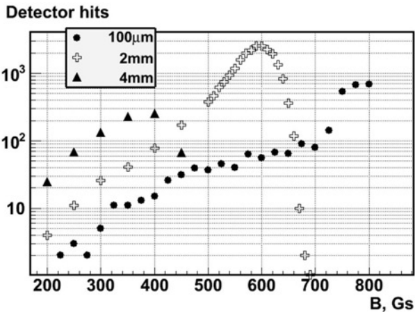
Figure 7. Magnetic field scans for different attenuator thickness.
