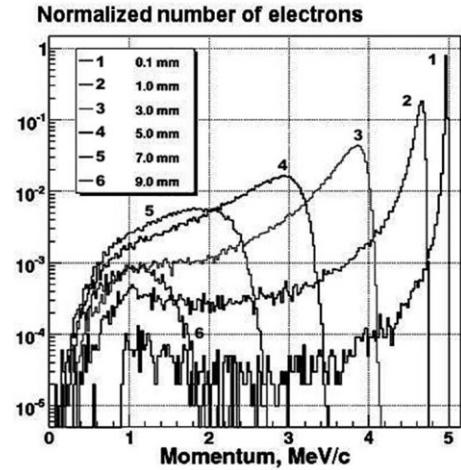
Figure 5. Momentum spectra of electrons after passing the Aluminum attenuators of different thickness. Momentum of primary electrons is 5 MeV/c
