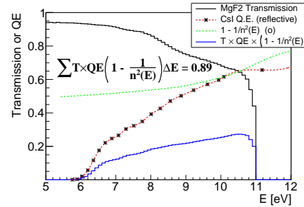
Figure 2. Transmission, refractive index of MgF 2 and quantum efficiency of CsI in reflective mode which were used for the calculation of the number of photoelectrons.
