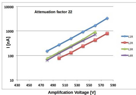
Figure 6. Current [nA] as a function of the amplification voltage [V] for the four layers of the MMSW2 chamber using an attenuation factor of the order of 22 corresponding to an incoming photon flux of 3 MHz/cm 2 .
