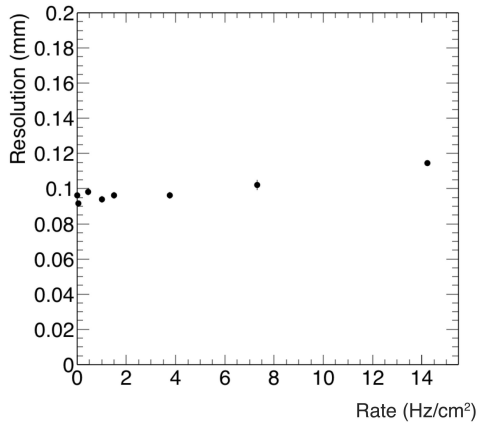
Figure 8. Resolution as a function of the incoming flux for L1 of MMSW2.
