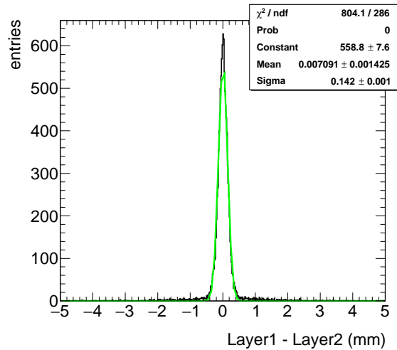
Figure 7. The distribution of the distance between the clusters on L1 and L2 for MMSW2 for the maximum flux, no attenuation factor. The fit is performed using a gaussian distribution function and the result of the fit is provided in the statistics box.
