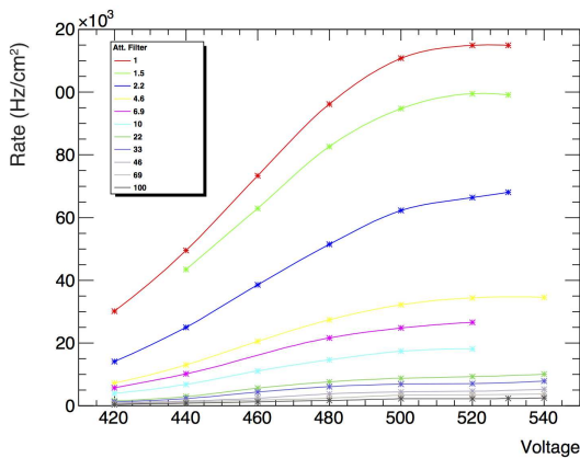
Figure 9. The measured particle rate as a function of the amplification voltage. The legend shows the different attenuation factors.
