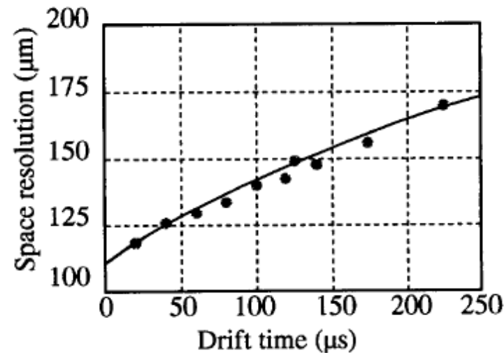
Fig. 20. Resolution in the drift time (350 V/cm). Curve is from described in
