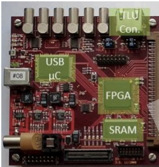
Multi-IO Board
