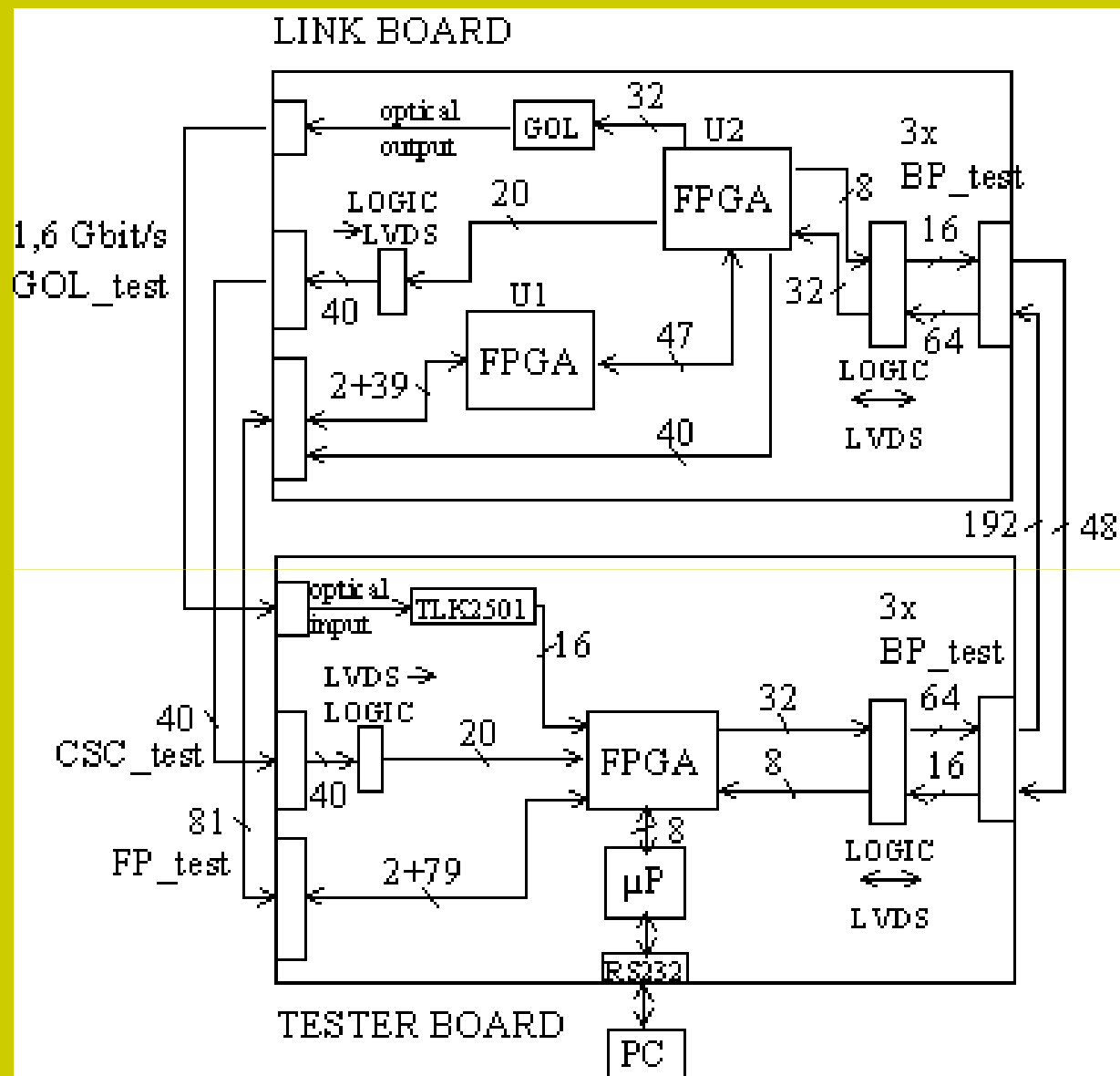
Signals and connections of the Link Board and the Tester Board.
