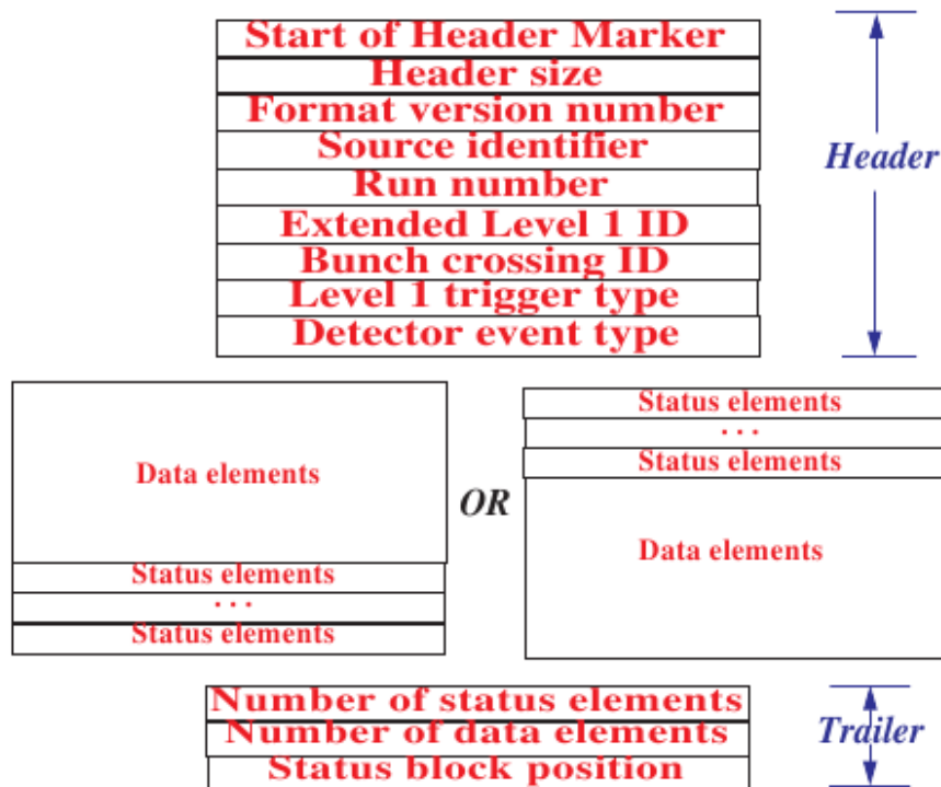
Figure 3: The ROD fragment format.
