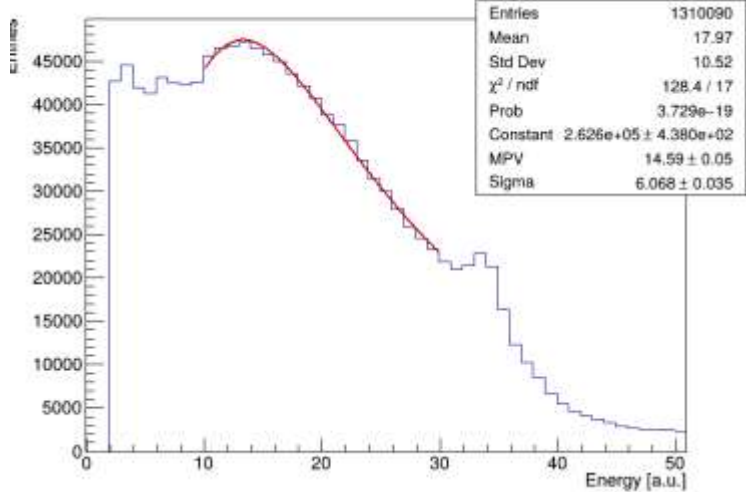
Strip Energy Y2
