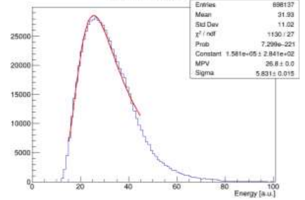
Cluster Energy Y3
