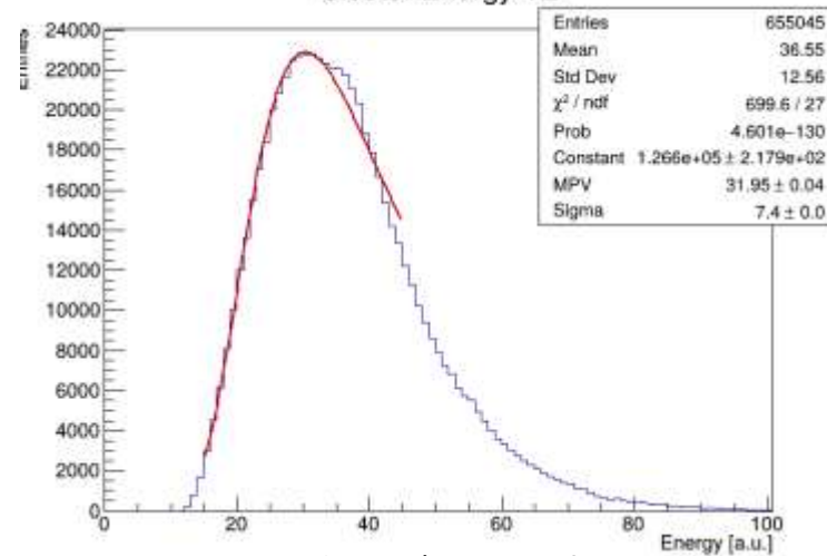
Cluster Energy Y2
