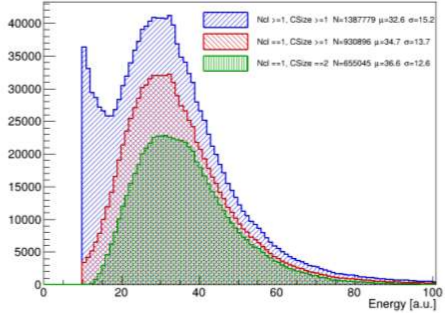
Cluster Energy Y2
