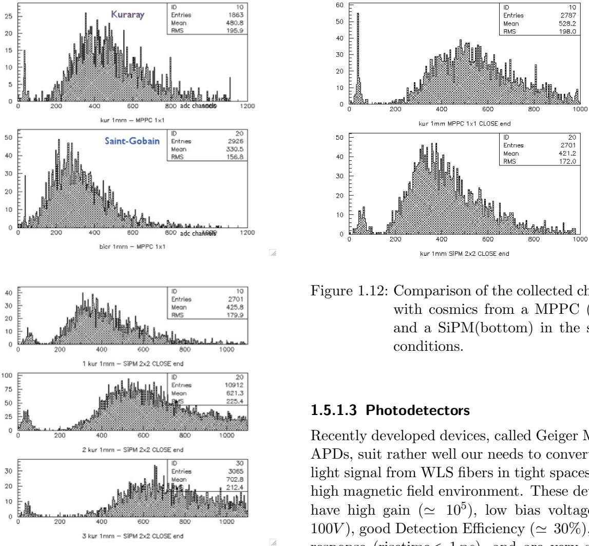
Figure 1.11: Top plot: light Yield for Kuraray Y11(top plot) and Saint-Gobain BCF92 (bottom plot) fibers. Bottom plot: comparison of the light yield of 1,2,3 fibers. All the above plots refers to data collected with cosmic rays.
