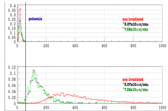
Figure 1.13: Comparison of the cosmic signal distribution before and after the irradiation, for a FBK 1 \text{ mm}^2 device.
