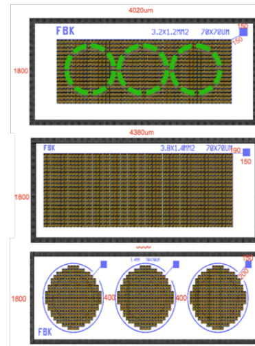
Figure 1.24: the custom SiPM manufactured by FBK for the IFR prototype
