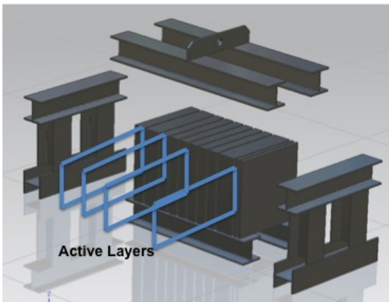
Figure 1.14: The IFR prototype.
