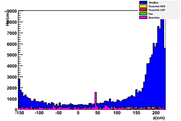
Figure 1.7: Photons Rate on IFR Barrel Layer 0 due to different background sources.
