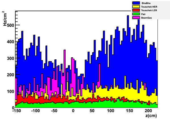
Figure 1.4: Neutron rate on IFR Barrel Layer 0 due to different background sources, the rates are normalized to 1 MeV equivalent [8] .
