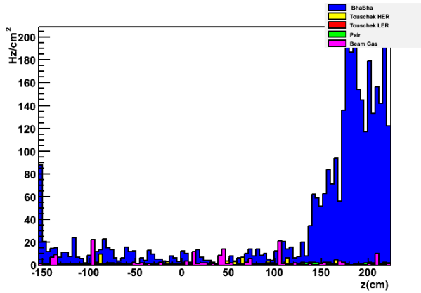
Figure 1.5: Electron rate for the IFR Barrel layer 0 due to different background sources the threshold for the deposited energy is *** MeV .
