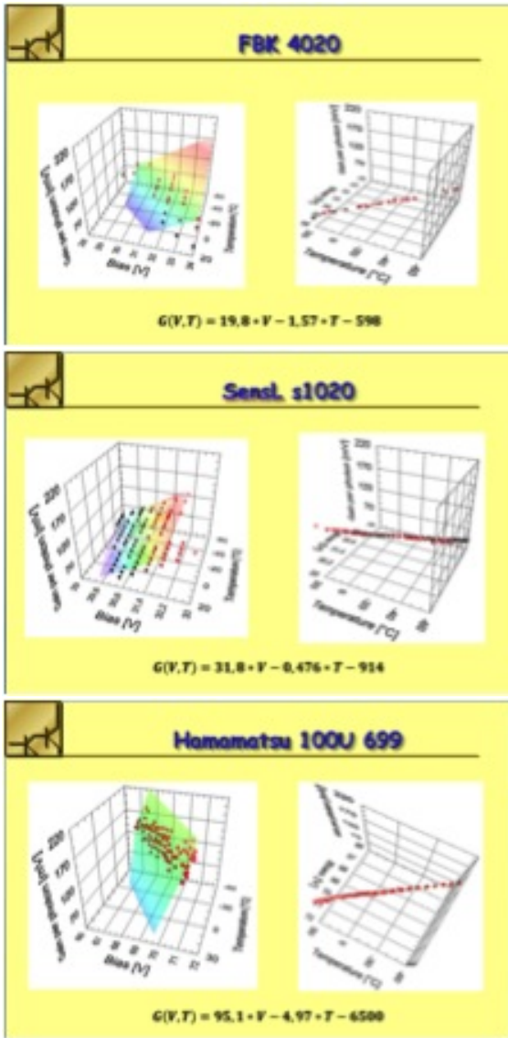
Figure 1.27: compensation of temperature fluctuation in SiPM's gain for FBK, SenSL and Hamamatsu devices.
