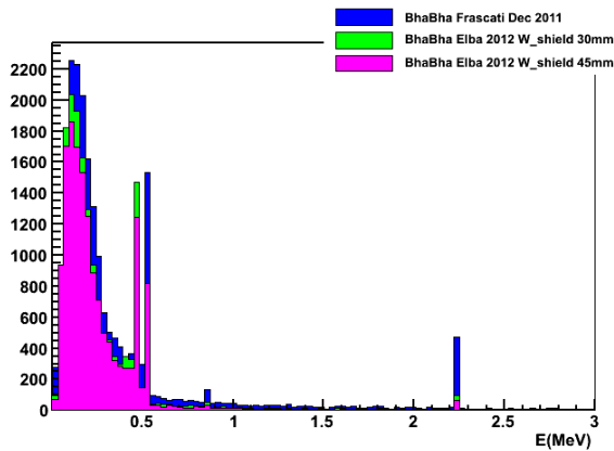
Figure 1.6: Photon energy spectrum for IFR Barrel Layer 0 .
