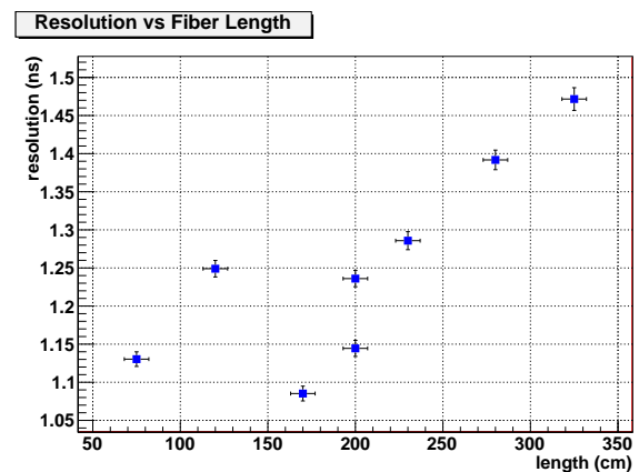
Figure 1.19: Time resolution as function of the fiber length.
