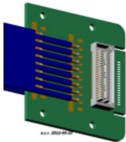
Figure 1.22: a detail of the multi coaxial connector assembly
