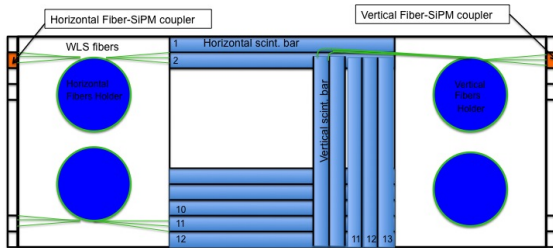
Figure 1.16: Scheme of an active module of the prototype.
