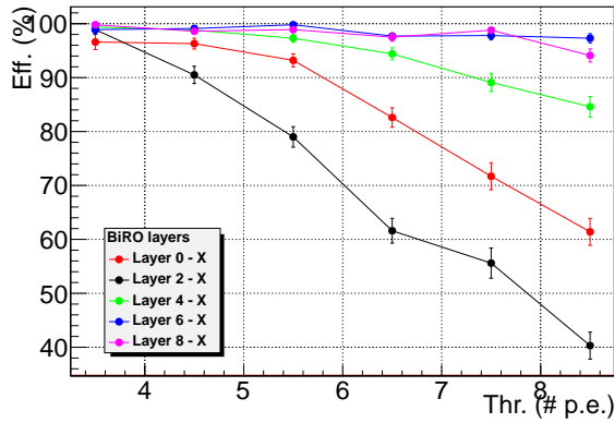
Figure 1.18: Prototype detection efficiency as function of the electronic threshold.
