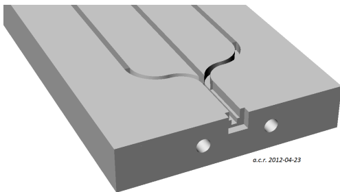
Figure 1.20: a scintillator bar machined to host three WLS fibers, the silicon photomultiplier and the carrier printed circuit board (PCB)
