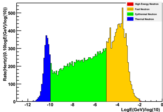
Figure 1.3: Neutron energy spectrum on IFR barrel, the neutron are classified according to their kinetic energy range as high energy neutron, fast, epithermal or thermal.
