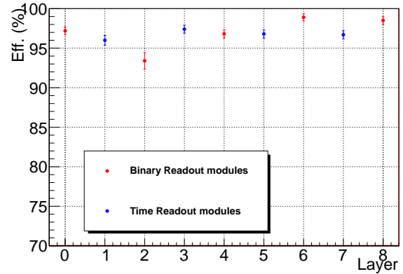
Figure 1.17: Prototype detection efficiency for each layer.
