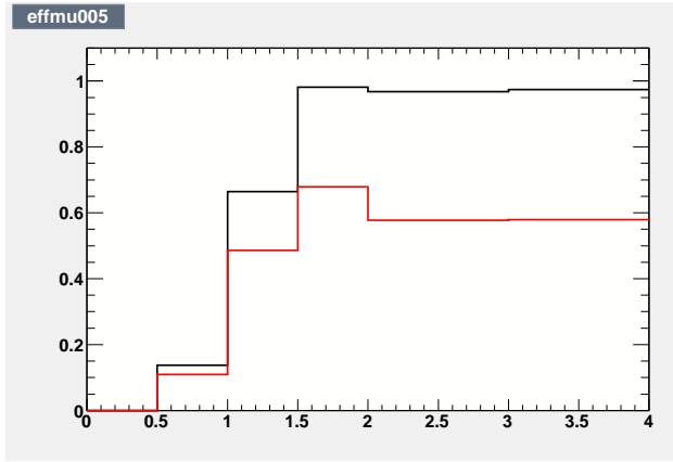
Figure 1.10: Muon efficiency as a function of the momentum, with \pi mis-id rate fixed in each momentum bin to be 2% (red) and 5% (black).
