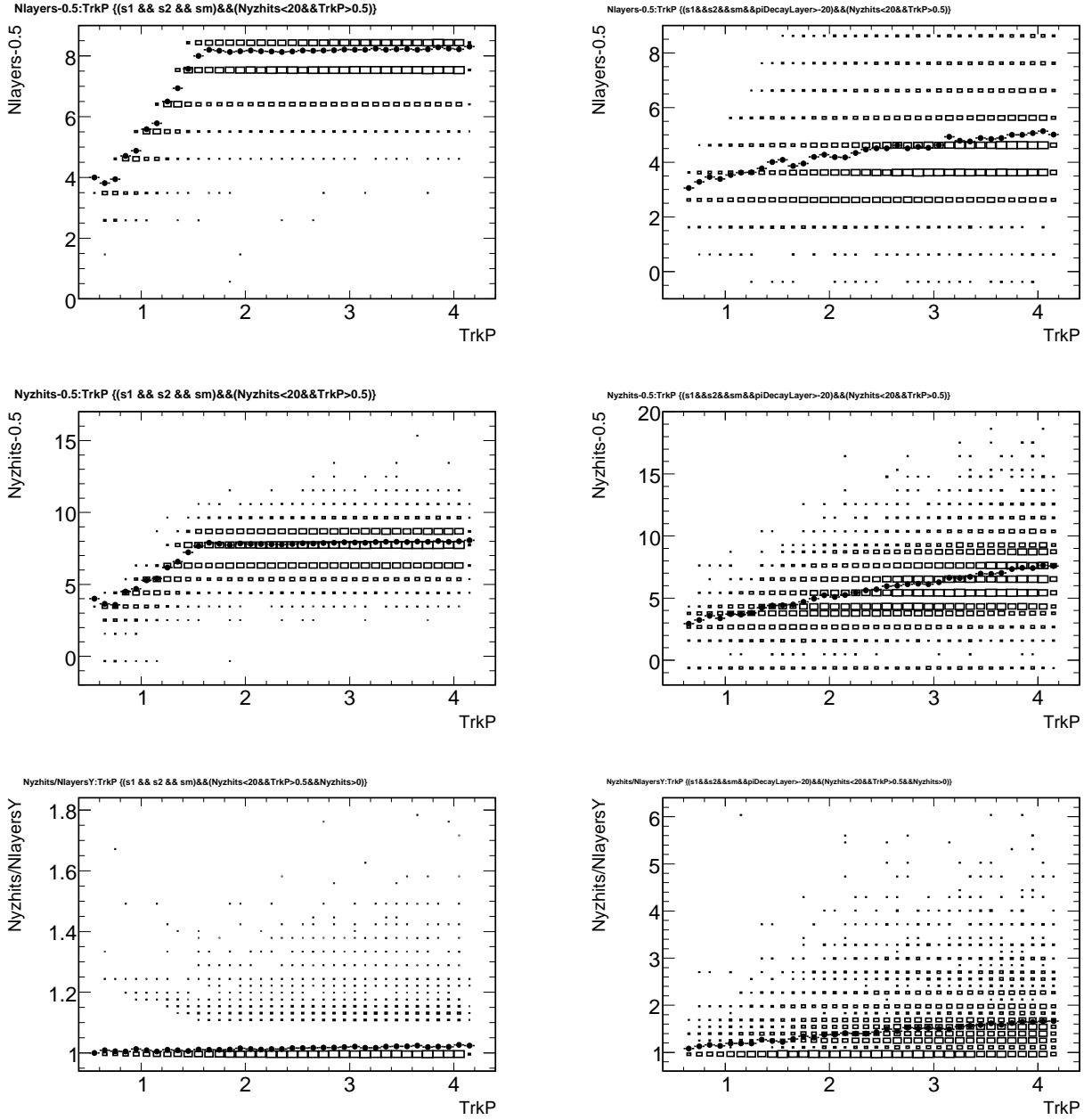
Figure 1.8: Distribution of the number of active layers, total number of hits and average number of hits per active layer, as a function of the particle momentum for \mu (left) and \pi (right). The dots represent the profile of the distribution.
