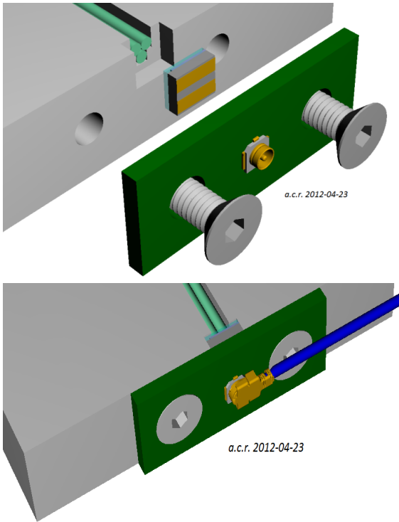
Figure 1.21: details of the three WLS fibers and the PCB for the solid state detector
