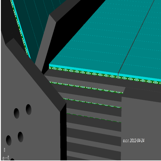
Figure 1.23: Location of the solid state detectors inside the IFR barrel: the detail shows IFR layer 0 detectors belonging to different modules (with the enclosure of the modules removed).
