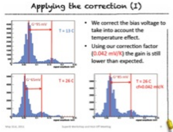
Figure 1.26: compensation of temperature-related SiPM gain shift by bias voltage adjustments
