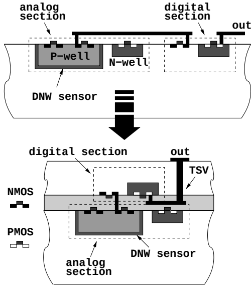
Figure 6.17: cross-sectional view of a DNW CMOS MAPS: from a planar CMOS technology to a 3D process
