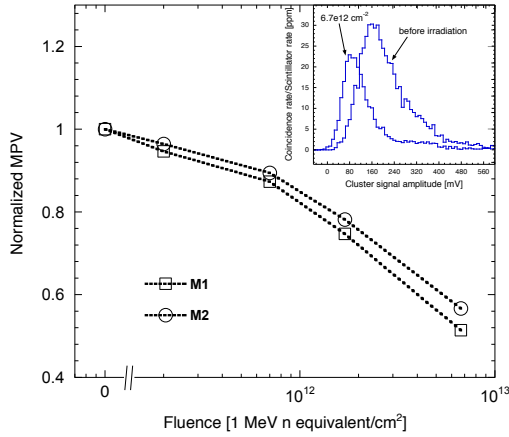
Figure 6.21: most probable value (MPV) of the ^{90}\text{Sr} spectra (shown in the inset for one of the tested chips before irradiation and after exposure to a 6.7 \times 10^{12} \text{ cm}^{-2} neutron fluence) normalized to the pre-irradiation value as a function of the fluence for DNW MAPS with different sensor layout.
