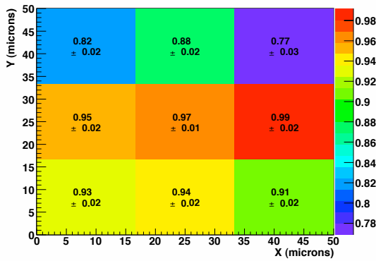
Figure 6.16: hit efficiencies measured as a function of position within the pixel (the picture, which is not to scale, represents a single pixel divided into nine sub-cells).
