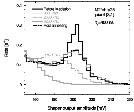
Figure 6.20: event count rate for a DNW monolithic sensor exposed to a ^{55}\text{Fe} source before irradiation, after exposure to \gamma -rays and after the annealing cycle.
