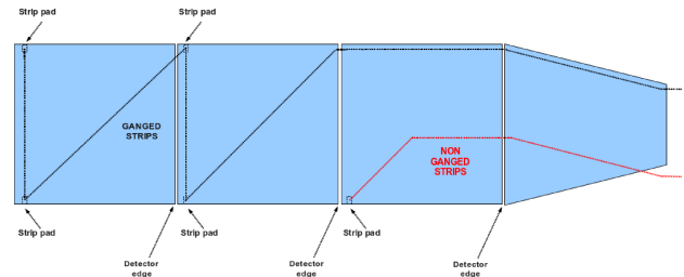
Figure 6.5: Schematic view of two z strips ganged through the fanout circuit.
