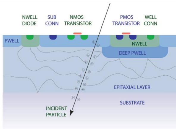
Figure 6.11: cross-sectional view of the INMAPS CMOS technology; emphasis is put on the deep P-well layer, rier to charge diffusing in the epitaxial layer,
