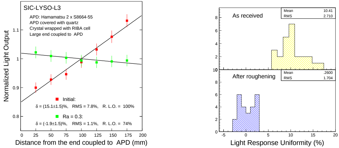
Figure 9.16: Left: Light response uniformity measured with two Hamamatsu S8664-55 APD readout for a tapered SuperB LYSO crystal SIC-L3 before (red dots) and after (green dots) uniformization by roughening the smallest side surface to R_a = 0.3 . Right: The distributions of light response uniformity ( \delta values) are shown for 25 SuperB test beam crystals before (top) and after (bottom) uniformization by roughening the smallest side surface.
