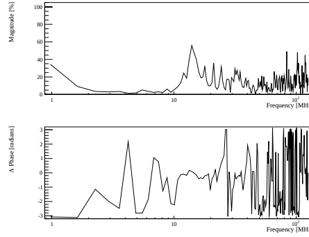
Figure 9.46: Correlation between crystals 2 and 10 as a function of the frequency. The phase takes random values when the magnitude is zero, when this happens its value should not be considered.
