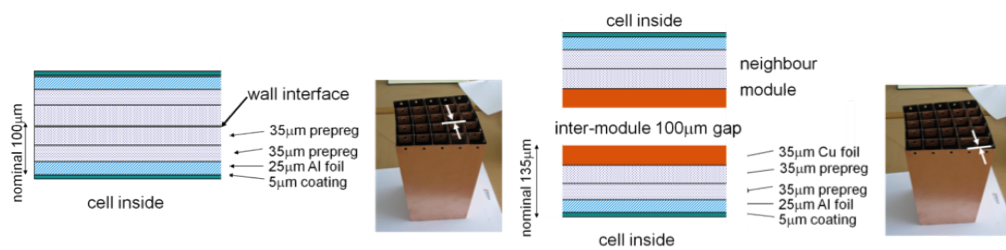
Figure 9.33: Alveolar module walls internal and external
