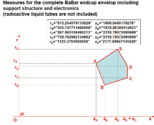
Figure 9.22: FWD EMC envelope.
