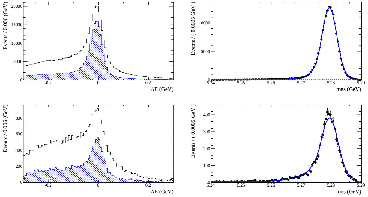
Figure 9.59: \Delta E (left) and m_{ES} (right) for B^- \rightarrow D^0 \pi^- with D^0 \rightarrow K^- \pi^+ \pi^0 reconstruction with both photons detected in the barrel and forward EMC (top) and one photon detected in the backward EMC (bottom). The two histograms in each \Delta E plot are before and after a D^0 mass cut.
