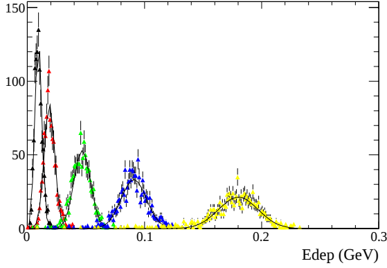
Figure 9.55: Energy depositions from mono-energetic photons (0.1 GeV, 0.2 GeV, 0.5 GeV, 1 GeV and 2 GeV) observed in the scintillators of the backward EMC generated in front of the EMC.
