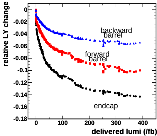
Figure 9.11: The light yield loss in the BABAR CsI(Tl) crystals due to radiation damage as a function of luminosity. The total dose received after 300\text{ fb}^{-1} is 1.2\text{ krad} in the endcap and 750\text{ rad} in the barrel.
