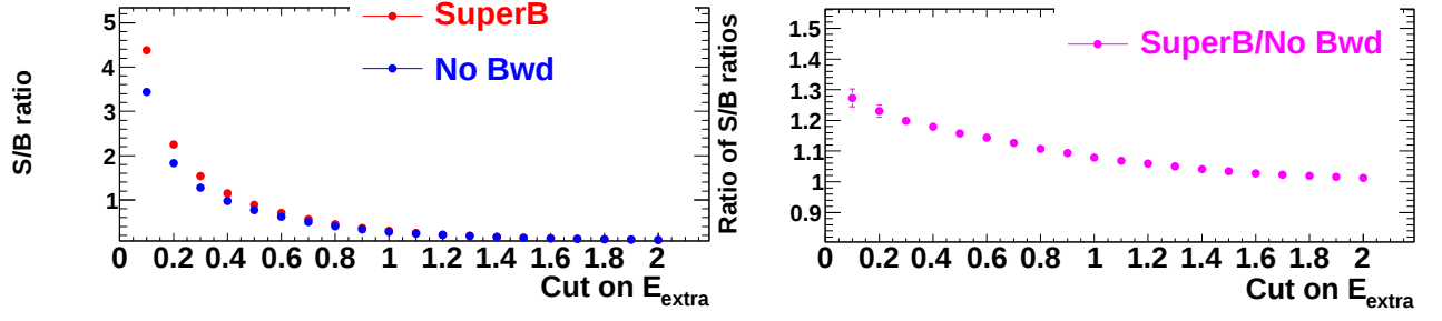
Figure 9.57: Left: Signal-to-background ratio with and without a backward EMC, as a function of the E_{\text{extra}} selection. Right: Ratio of the S/B ratio with a backward EMC to the S/B ratio without a backward calorimeter, as a function of the E_{\text{extra}} selection.
