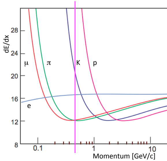
Figure 9.61: Calculated energy loss curves versus momentum for e , \mu , \pi , K and p in one layer of the backward EMC.
