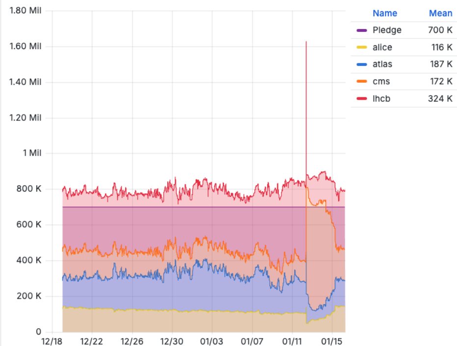
HEPScore usage LHC
