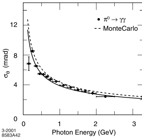
Figure 9.8: photon energy (top) and angular (bottom) resolution from Babar experiment.
