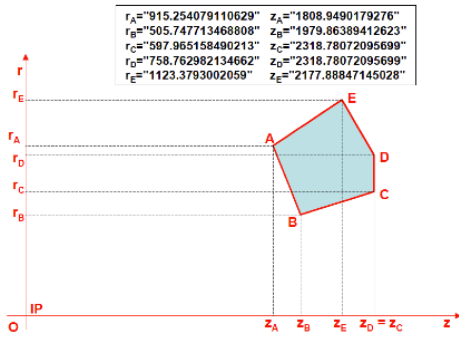
Figure 9.22: FWD EMC envelope.
