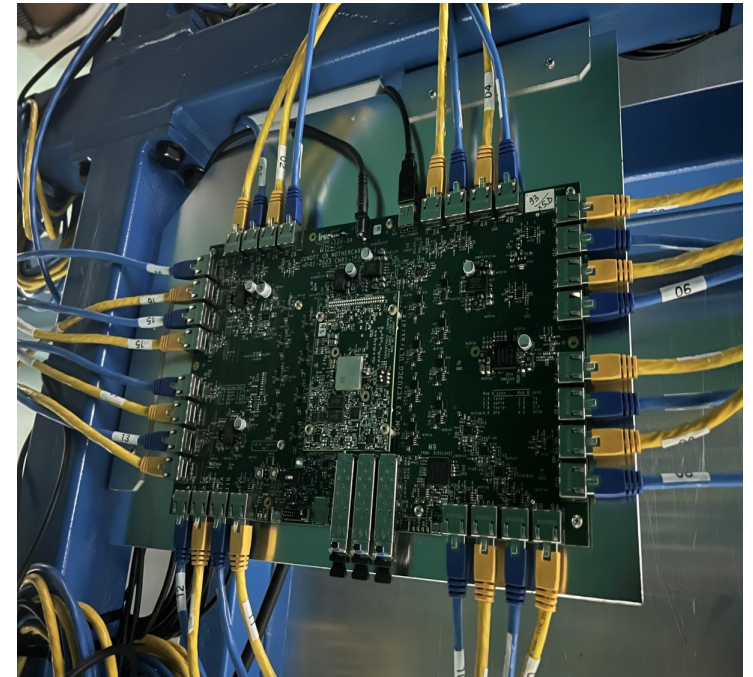
Concentrator
