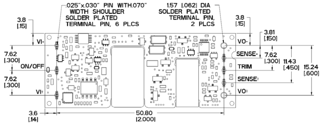
Bottom View
