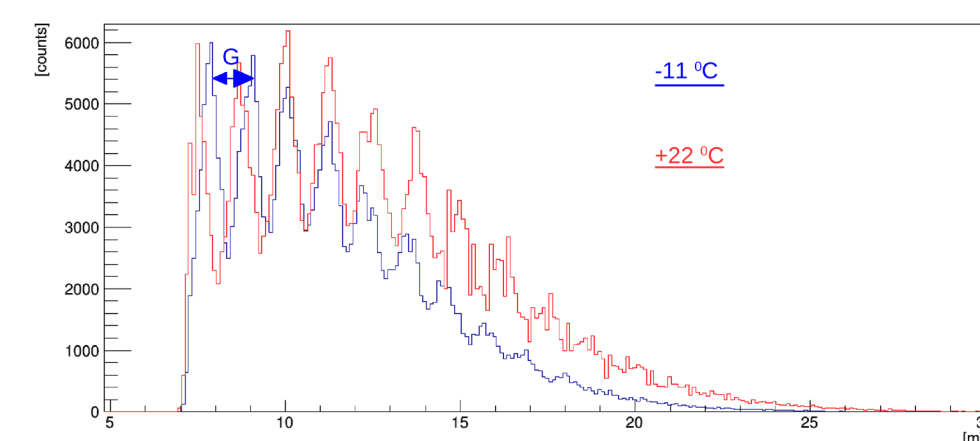
d) Typical charge distribution of SiPM illuminated by pulsed LED 400 nm light. It shows a constant gain in the interval T = 22^\circ\text{C} (red) to -11^\circ\text{C} (blue).
