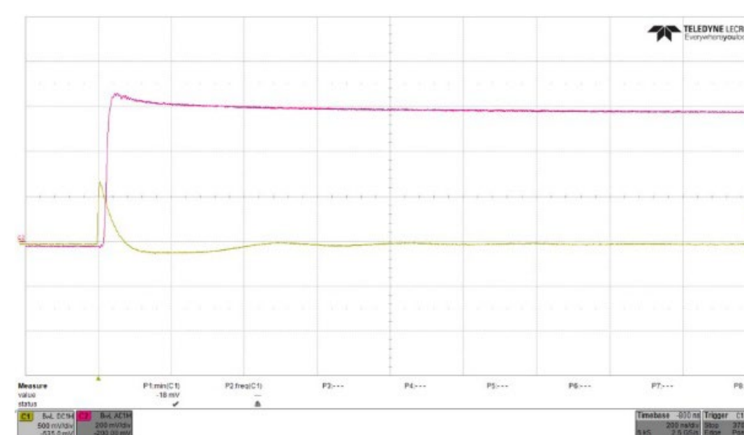
Figure 5: SiPM signal (yellow) and the peak-hold output (red). The scope setup is 200 ns/div and 500 mV/div for the SiPM signal and 200 mV/div for the peak-hold output signal.
