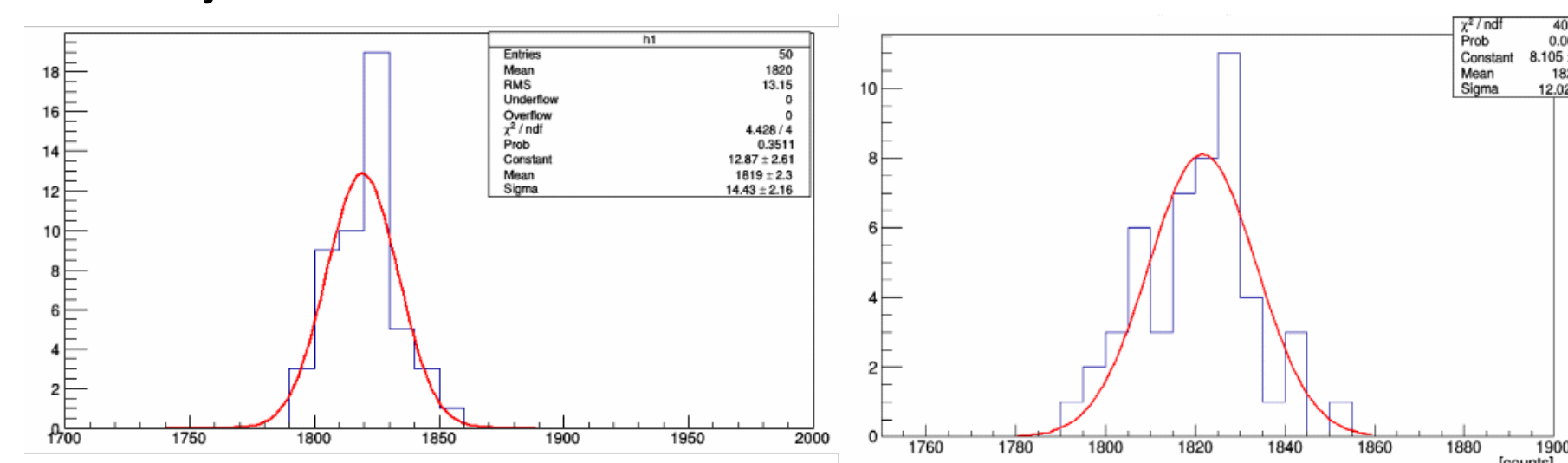
Figure 3. Left: The Gaussian fit of the averaged integral values over nine hours. Right: The Gaussian fit of the averaged integral values over 100 s with 10 s step.
