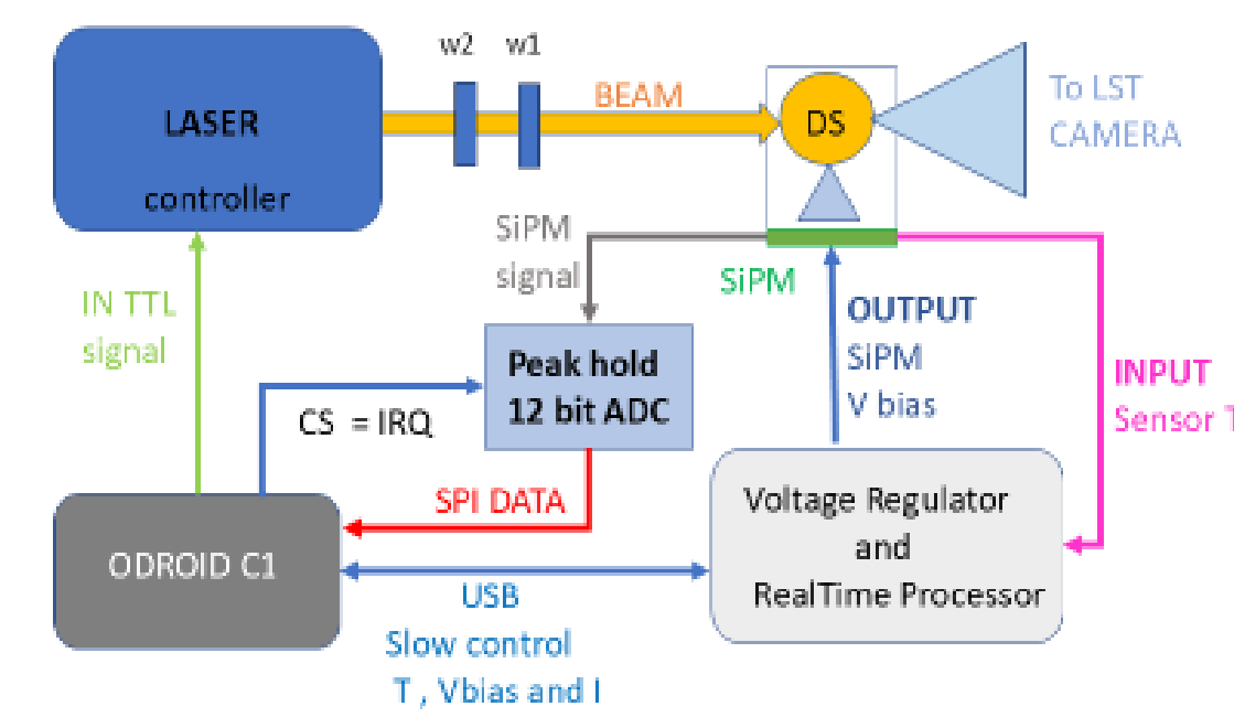
Figure 6: Block diagram of the system to monitor the photon flux sent to the camera with all details. In the figure DS = diffusing sphere. The ODROID starts the laser via a TTL signal sent via GPIO; the ADC uses a dedicated peak and hold circuitry and a delayed TTL IRQ signal from the Odroid to measure the SiPM signal charge. The Voltage regulator senses the temperature near the SiPM and adjusts, according to a calibrated linear function, the bias Voltage of the SiPM to maintain the gain constant with changing temperatures.
