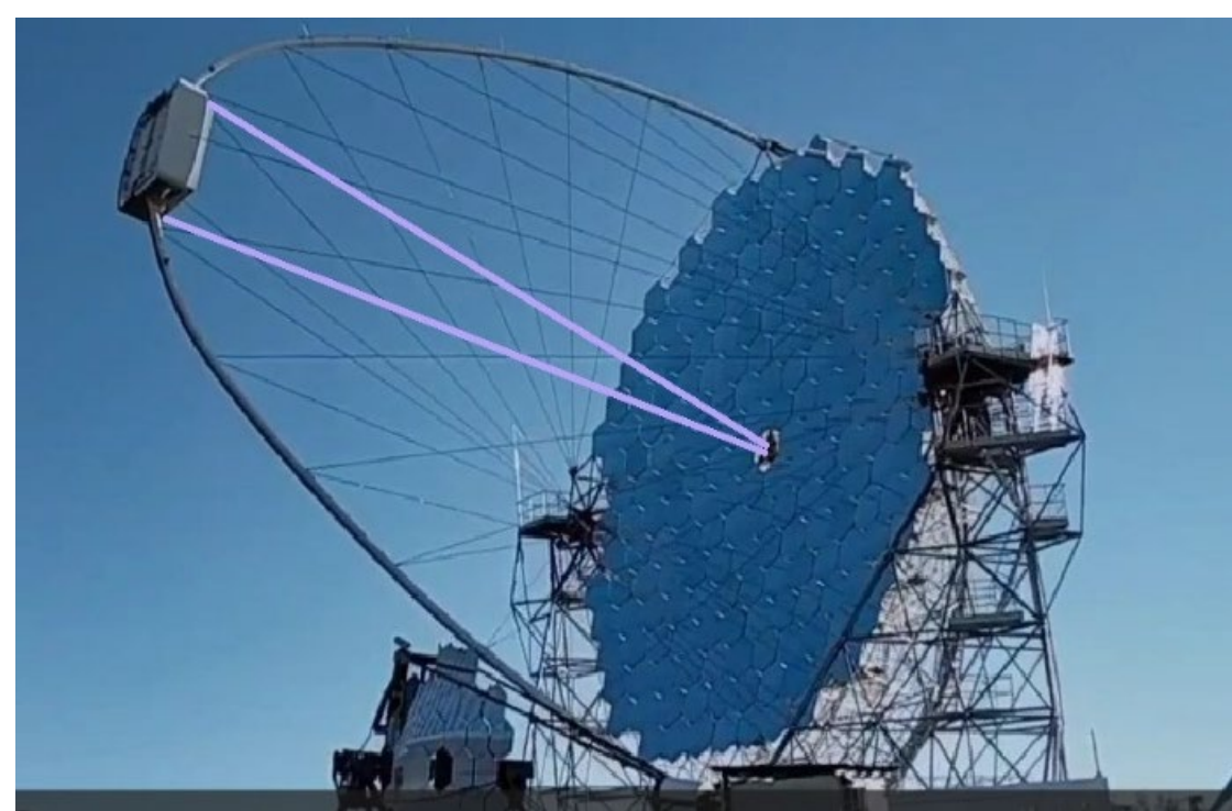
Fig. 2 LST-1. The CaliBox is installed in the center of the dish.
