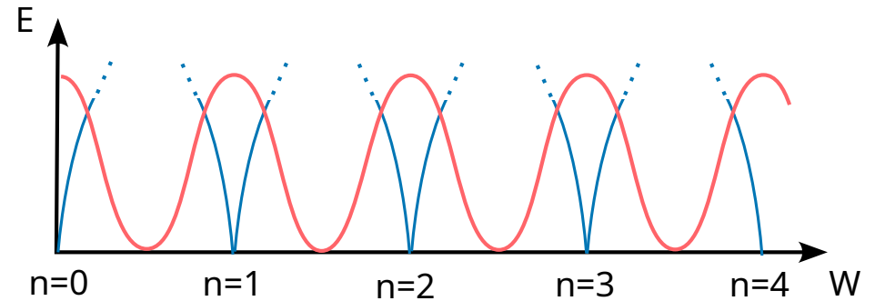
QM expectation
