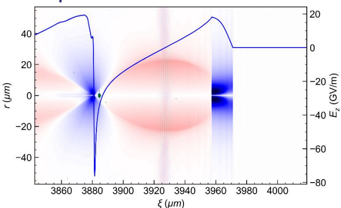
fbpic simulation
