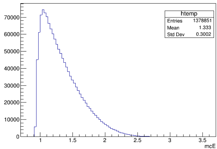
mcE {mcPDG==22}
