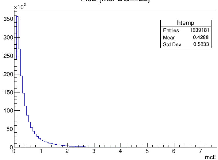
mcE {mcPDG==22}
