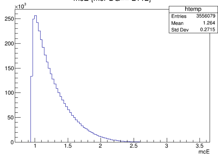
mcE {mcPDG==2112}
