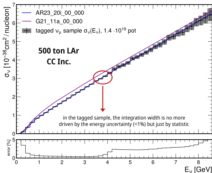
CC \nu_\mu cross section
