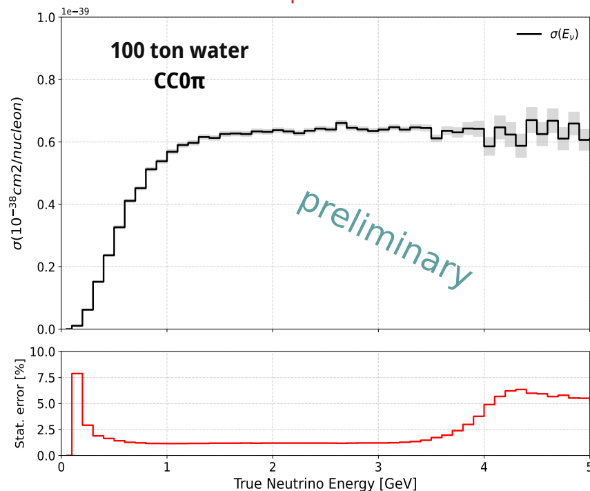
CC0 \pi \nu_\mu cross section
