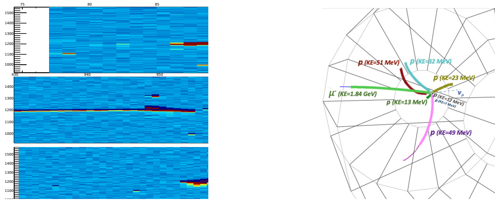
Fig. 5.: The same CC \nu_\mu event with seven low energy protons (kinetic energies ranging from 7 to 51 MeV) simulated in a LArTPC (left) and a HPgTPC (right). The LArTPC event display shows time ticks versus channel number for the three projective views of the event. The HPgTPC reconstruction algorithm finds all eight tracks in the event (seven proton tracks and one muon track), although only six are visible by eye in this view. All proton tracks travel 2.4 cm or less in LArTPC [6].
