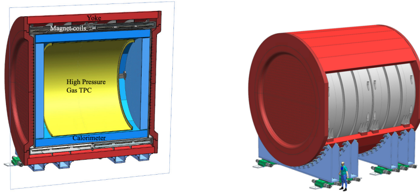
Fig. 4.: (Left) Cutaway view of the full ND-GAr detector system, showing the HPgTPC, the calorimeter, the magnet, and the iron yoke. The detectors for the muon-tagging system are not shown. (Right) The SPY magnet system. The hole in the yokes is on the upstream side, to minimize material traversed by tracks originating from neutrino interactions in ND-LAr [6].
