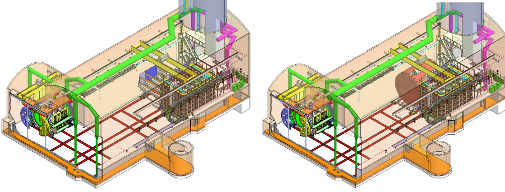
Fig. 1.: Layout of the envisaged Phase I (left) and Phase II (right) ND suite. The neutrino beam enters from the bottom-right corner, and exits at the top-left corner, of the drawings. The SAND detector is shown at its permanent on-axis location, while all other detectors upstream are shown at their maximum off-axis location [6].
