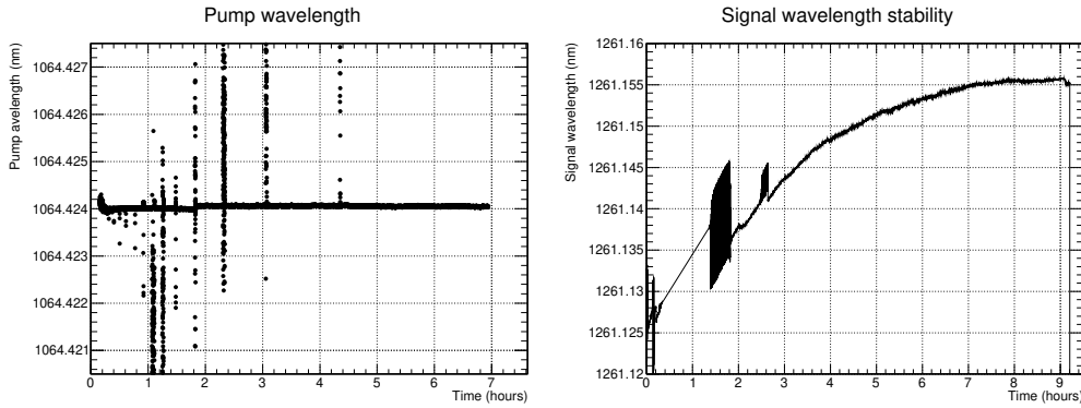
Fig. 2. – The two plots show the wavelength behavior of the pump and signal lasers during the initial hours after startup. On the left, the pump wavelength becomes nearly stable after the second hour, with rapid vertical fluctuations occurring alongside temporary losses of single-mode operation, which gradually subside over time. On the right, the signal wavelength exhibits a pronounced drift that stabilizes after approximately 7 hours, primarily due to temperature variations in the laser during startup.
