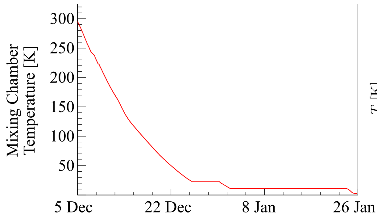
CUORE cryostat cooldown
