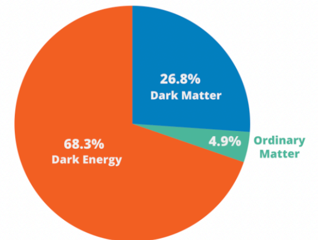
Estimated matter-energy content of the Universe
