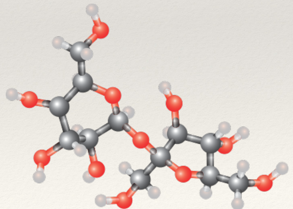
Molecola
