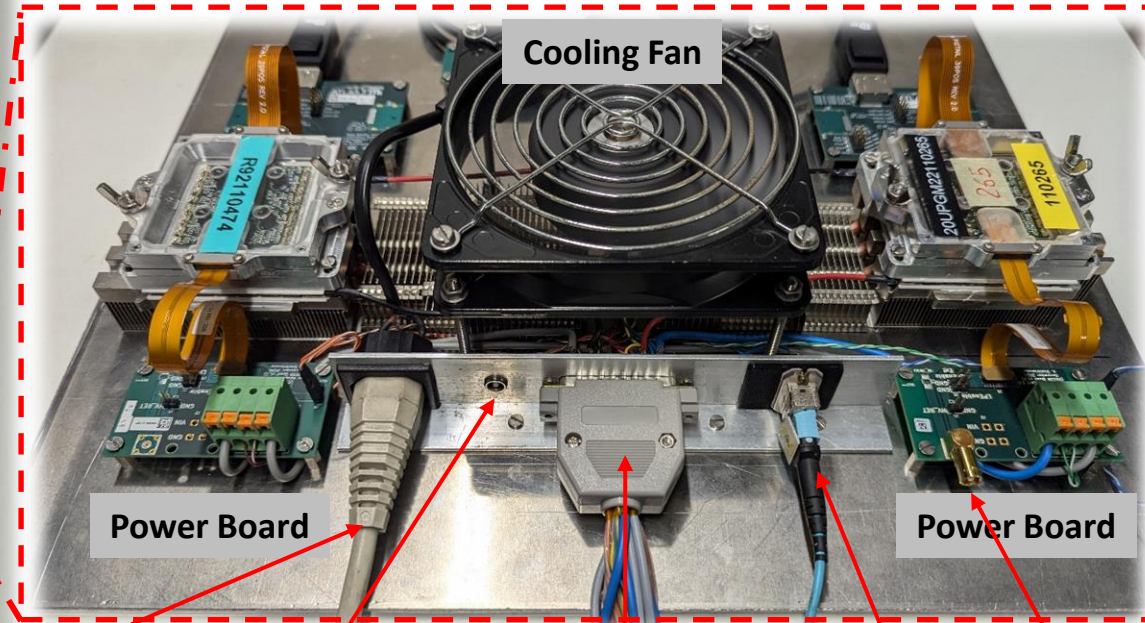
Fan Power LP Mode pulser Power Connector Optic Fibers HV
