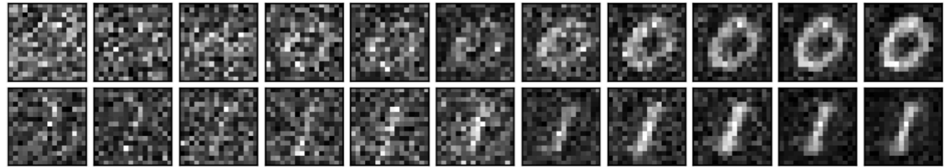
Denoising steps (quantum-hardware-oriented model)
