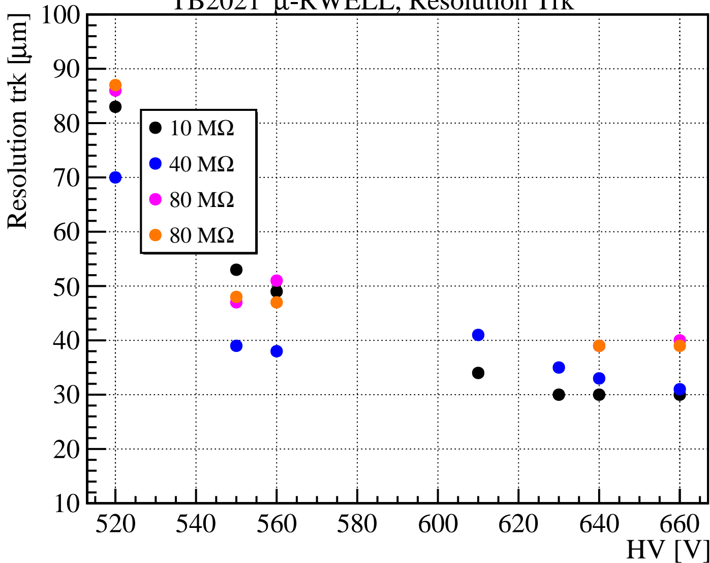
TB2021 \mu -RWELL, Resolution Trk
