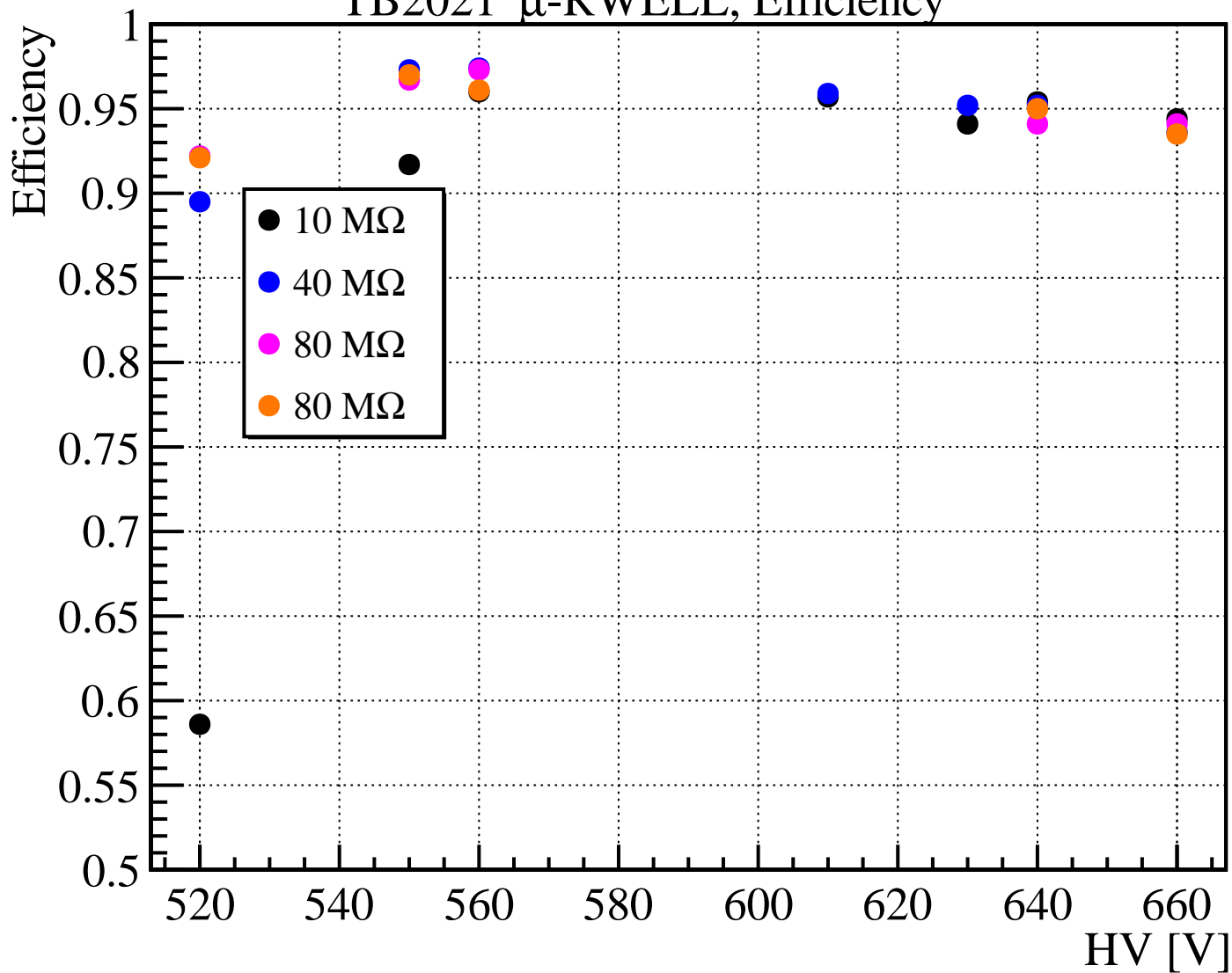
TB2021 \mu -RWELL, Efficiency
