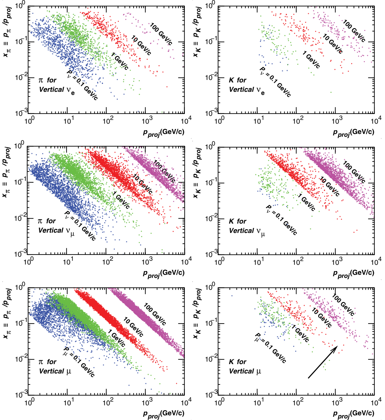
FIG. 1 (color online). The scatter plot of \pi 's ( \pi^+ and \pi^- , left) and K 's ( K^\pm , K_L^0 , and K_S^0 , right) in the phase space ( p_{\text{proj}}-x plane) at their production relevant to atmospheric \mu 's and \nu 's at the momenta, 0.1, 1.0, 10, and 100 GeV/c, at sea level for vertical directions. Here, x is defined as x \equiv p_m/p_{\text{proj}} in the rest frame of Air nuclei for m = \pi or K . We sampled 3000 \mu 's and 3000 \nu 's ( \nu_e + \nu_\mu ) at each momentum from the HKKM04 calculation. The arrow in the right bottom panel shows the directions to which p_{\pi,K} increase.
