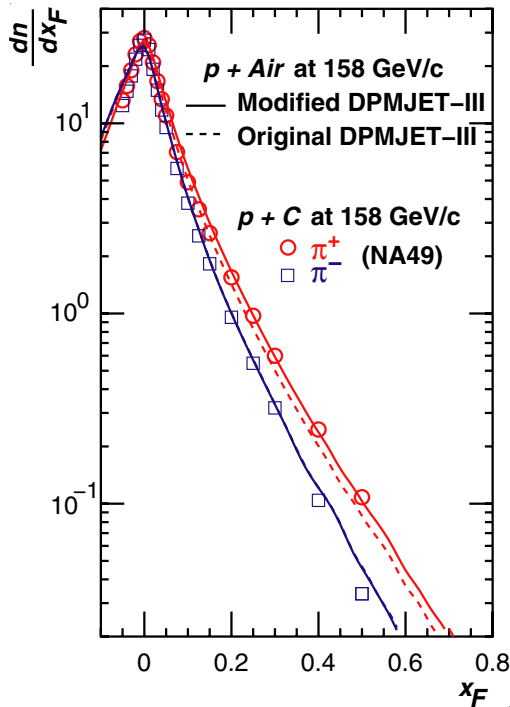
FIG. 15 (color online). The comparison of the \pi 's production spectra of the original and modified DPMJET-III in p + \text{Air} interaction with that in p + C from the NA49 experiment at 158 GeV/c. Note, the production spectrum of \pi^- of the modified DPMJET-III at 158 GeV/c is almost the same as that of the original DPMJET-III.
