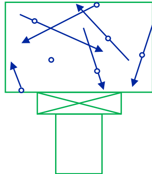
Molecular Flow (molecules move independently)
