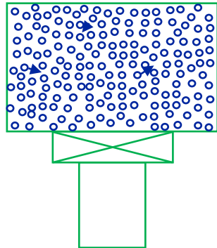
Viscous Flow (momentum transfer between molecules)
