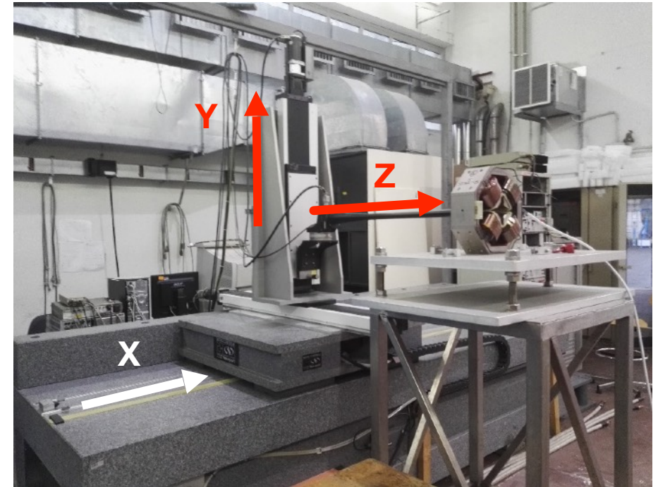
Coordinatometer
