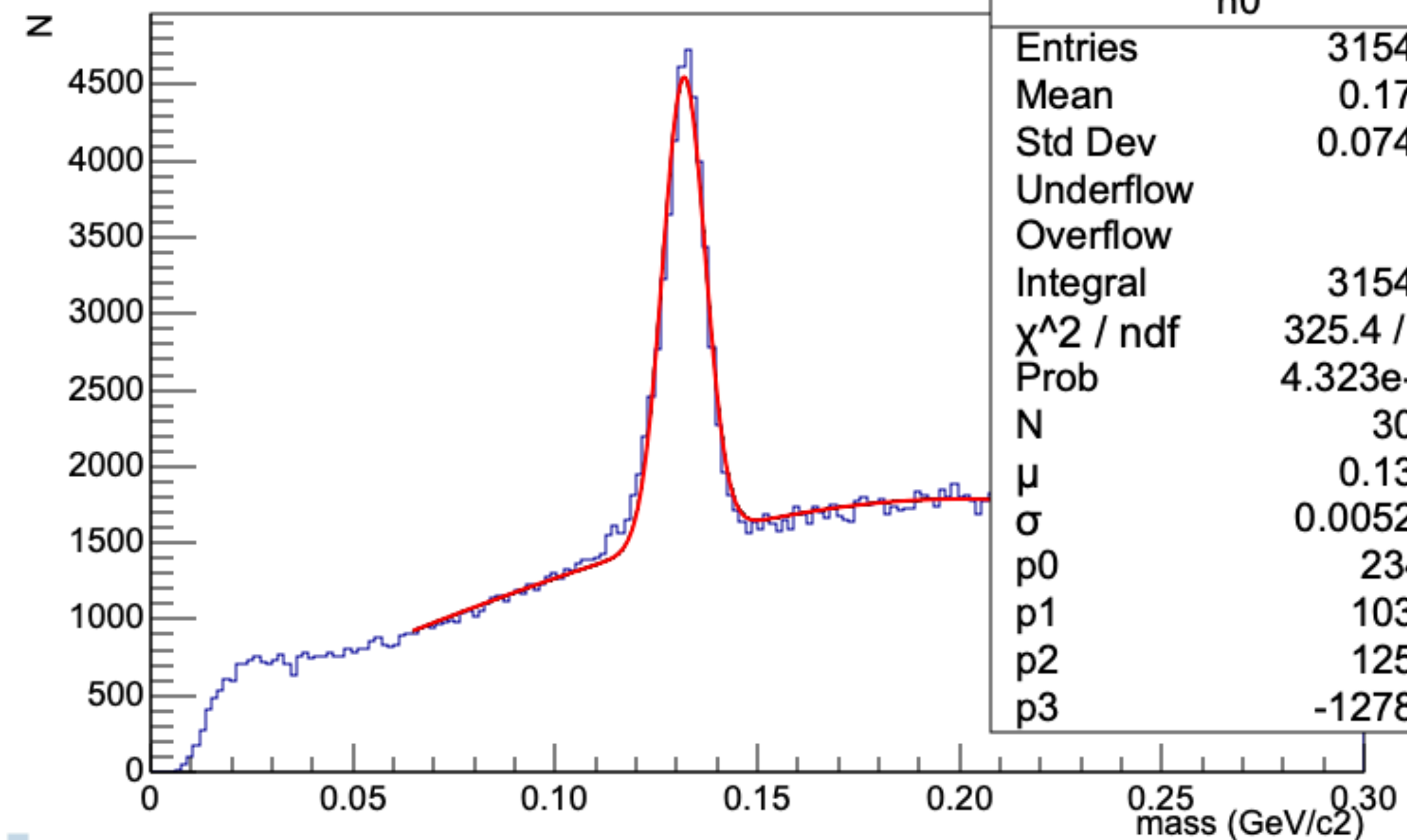
pi0 Invariant Mass Distribution
