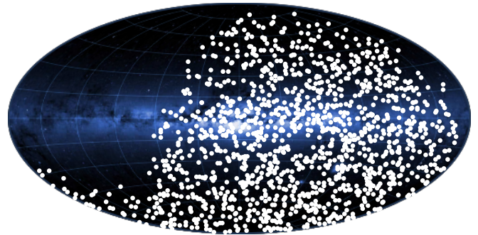
Galactic
