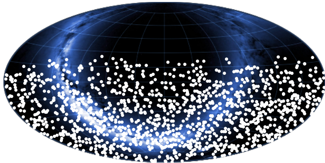
Equatorial
