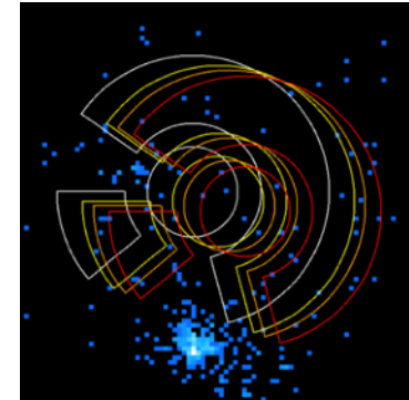
NuSTAR X-rays observations of the Sun
