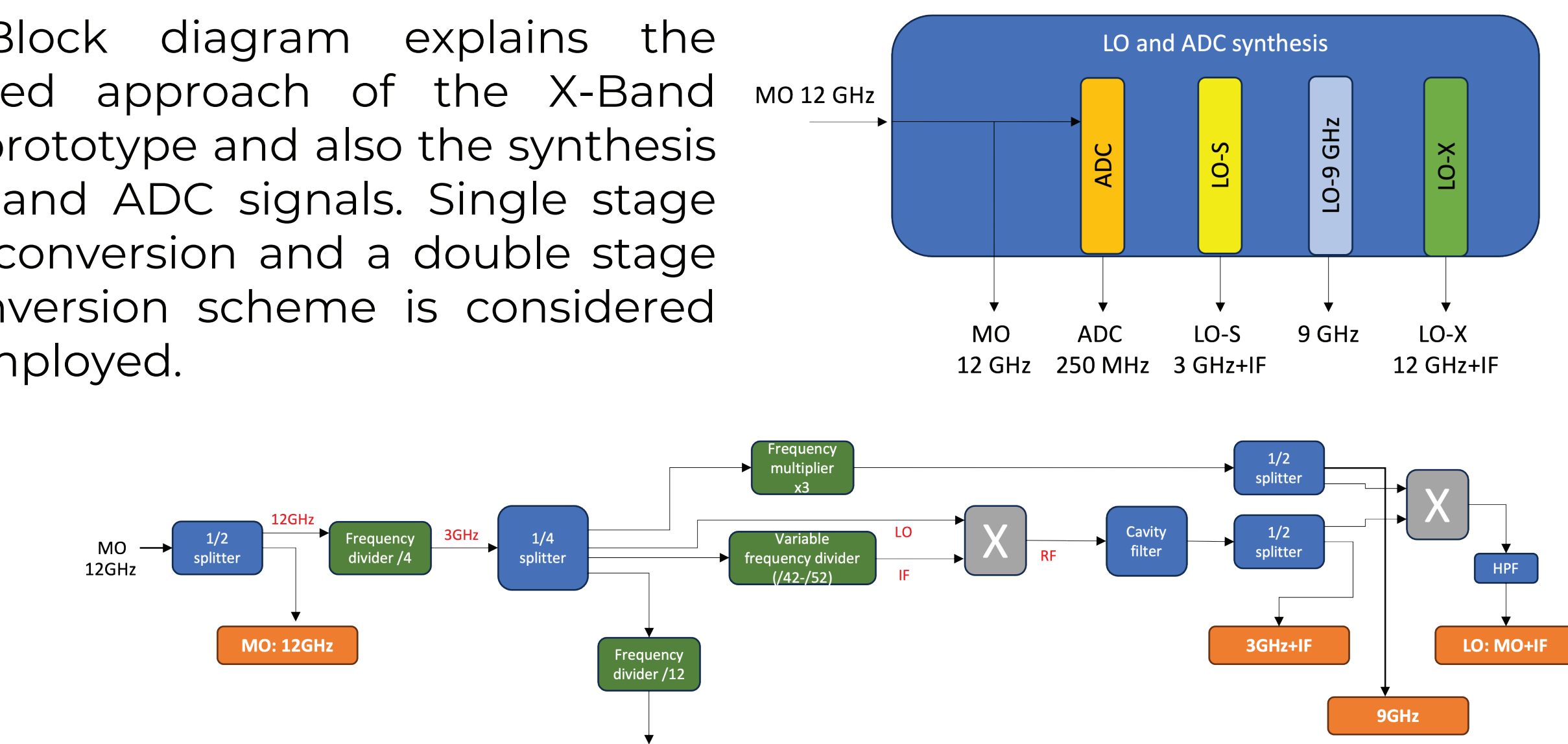
Figure 4: Architecture of LO and ADC synthesis block
