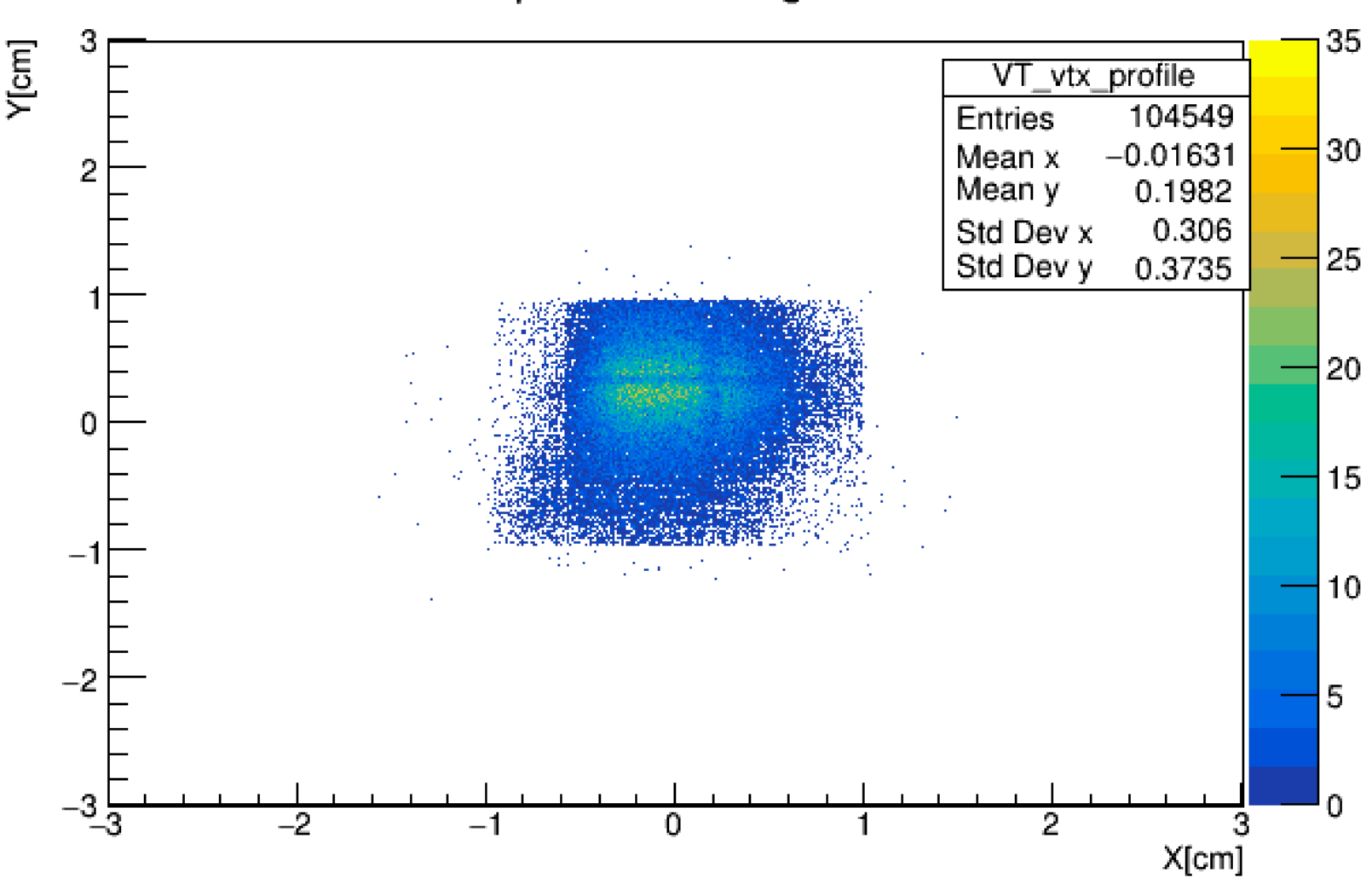
VTX profile on target
