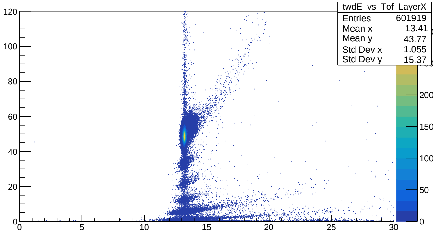
dE_vs_Tof_LayerX
