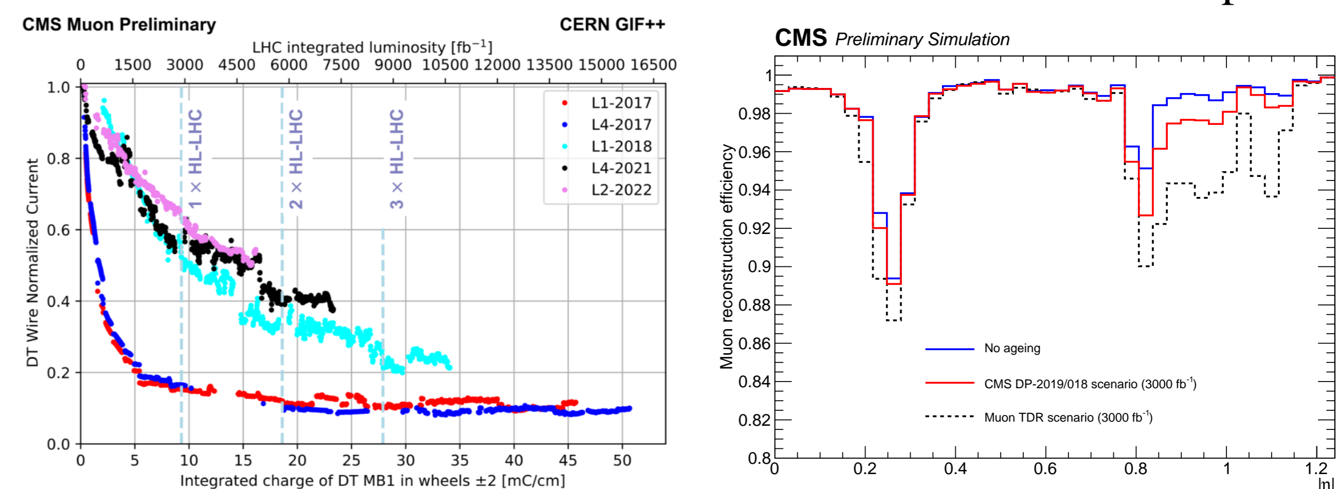
Figure 5: LEFT: Normalized current for different sets of irradiated wires as function of the integrated charge (dose). RIGHT: Muon reconstruction efficiency at CMS as a function of absolute \eta for non-aged DT chambers and aged DT chambers. The efficiencies have been calculated using simulated sample of dimuon events.
