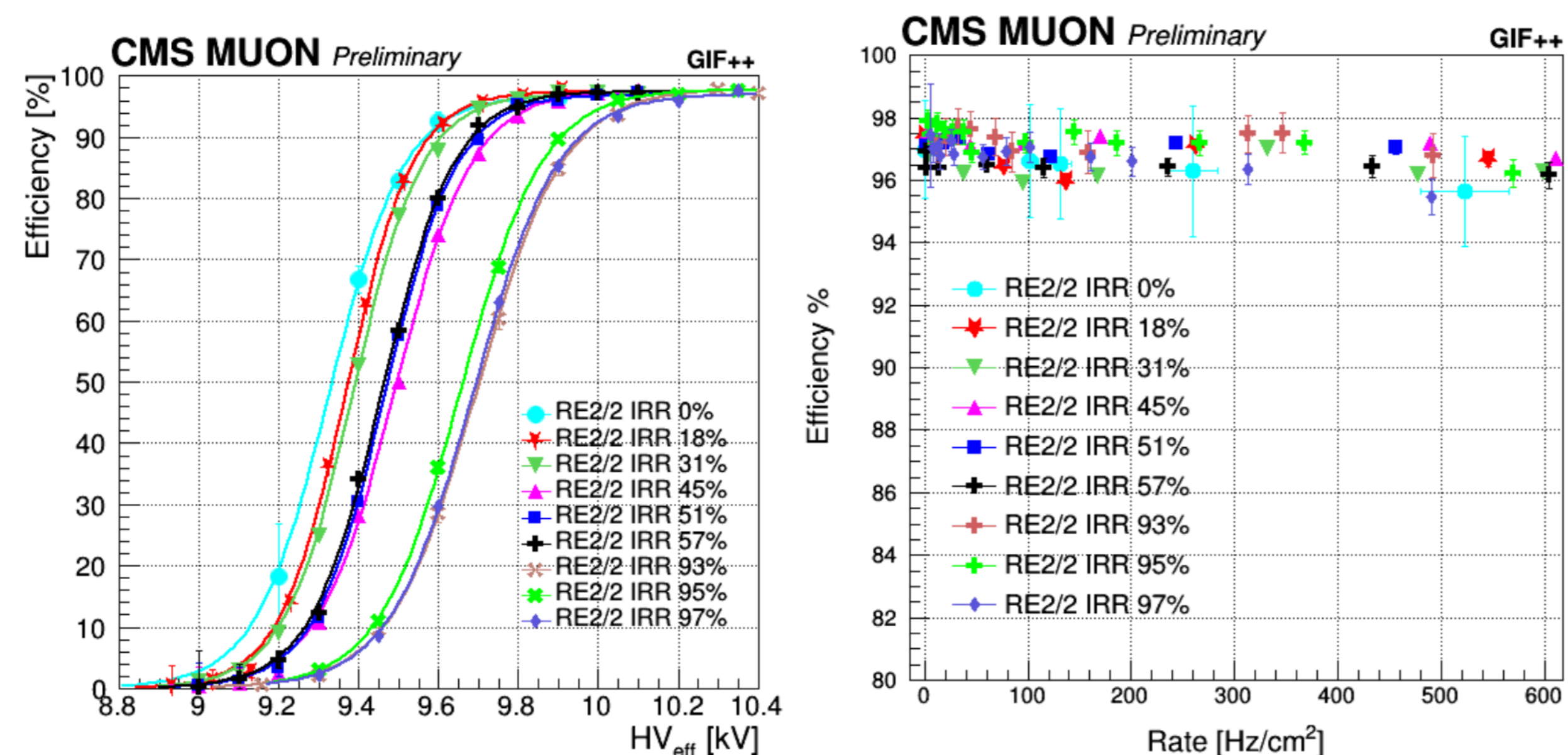
Figure 3: LEFT: RE2/2 irradiated chamber efficiency measured as a function of the effective high voltage, under a gamma background rate of about 600 Hz/cm 2 which represents the expected background rate at HL-LHC phase including safety factor of 3. RIGHT: RE2/2 irradiated chamber efficiency measured at the detector working point as a function of the background rate at different values of collected integrated charge.
