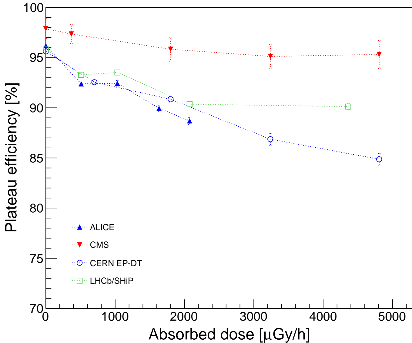
Plateau Efficiency vs. Dose with ECO3 mixture
