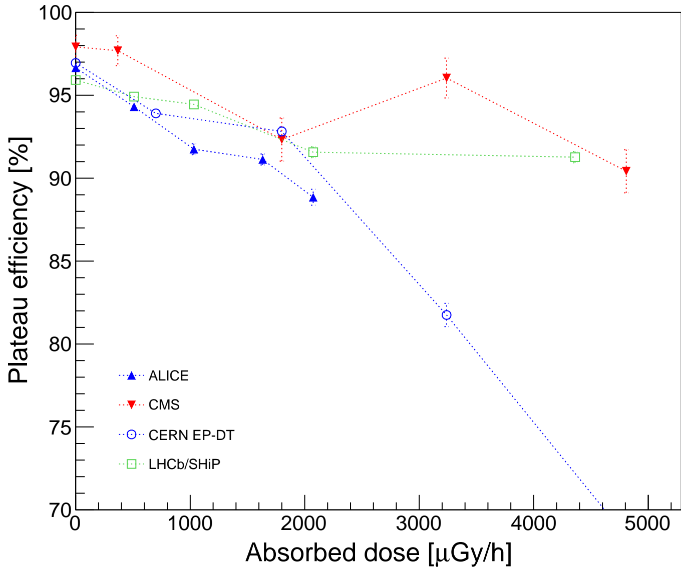
Plateau Efficiency vs. Dose with ECO2 mixture
