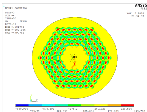
Figure 18: tensile test - \sigma_{eqv} , \sigma_{rr} , \sigma_{\theta\theta} , \sigma_{zz} at 0% load and 4.2K with residual stress
