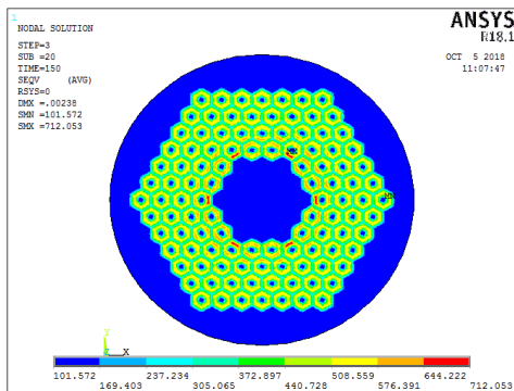
Figure 15: tensile test - \sigma_{eqv} , \sigma_{rr} , \sigma_{\theta\theta} , \sigma_{zz} at 0% load and 4.2K without residual stress
