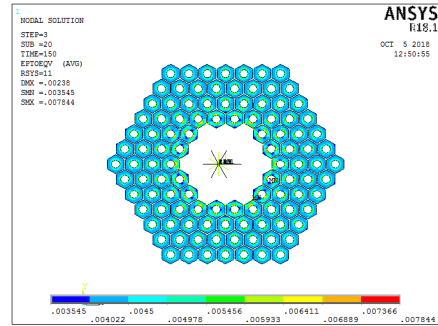
Figure 17: tensile test - equivalent strain in Nb 3 Sn at 0% and 100% load and 4.2K with residual stress
