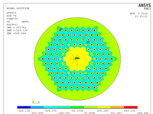
Figure 18: tensile test - \sigma_{eqv} , \sigma_{rr} , \sigma_{\theta\theta} , \sigma_{zz} at 0% load and 4.2K with residual stress
