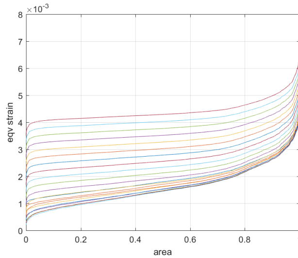
Figure 2: equivalent strain (function of area) in the strand cross section with increasing values of applied axial strain without the effect of residual stress
