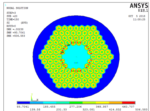
Figure 16: tensile test - \sigma_{eqv} , \sigma_{rr} , \sigma_{\theta\theta} , \sigma_{zz} at 100% load and 4.2K without residual stress
