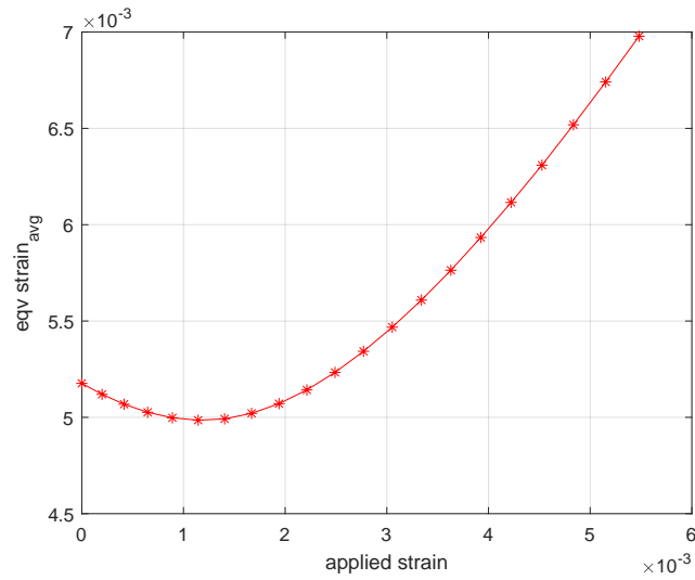
Figure 5: average equivalent strain in the strand's cross section as a function of the applied axial strain value with the effect of residual stress
