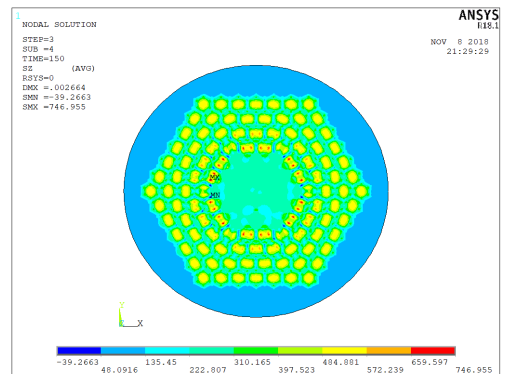
Figure 19: tensile test - \sigma_{eqv} , \sigma_{rr} , \sigma_{\theta\theta} , \sigma_{zz} at 100% load and 4.2K with residual stress
