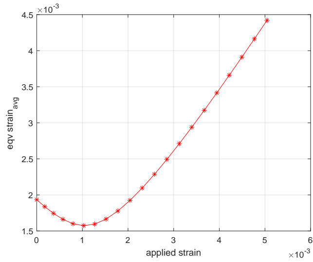
Figure 3: average equivalent strain in the strand's cross section as a function of the applied axial strain value without the effect of residual stress
