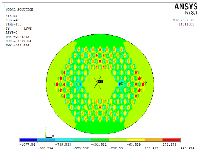
Figure 21: tensile test - \sigma_{eqv} , \sigma_{xx} , \sigma_{yy} , \sigma_{zz} at 0% load and 4.2K with residual stress
