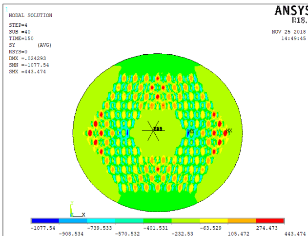
Figure 22: tensile test - \sigma_{eqv} , \sigma_{xx} , \sigma_{yy} , \sigma_{zz} at 100% load (external pressure = 200Mpa) and 4.2K with residual stress
