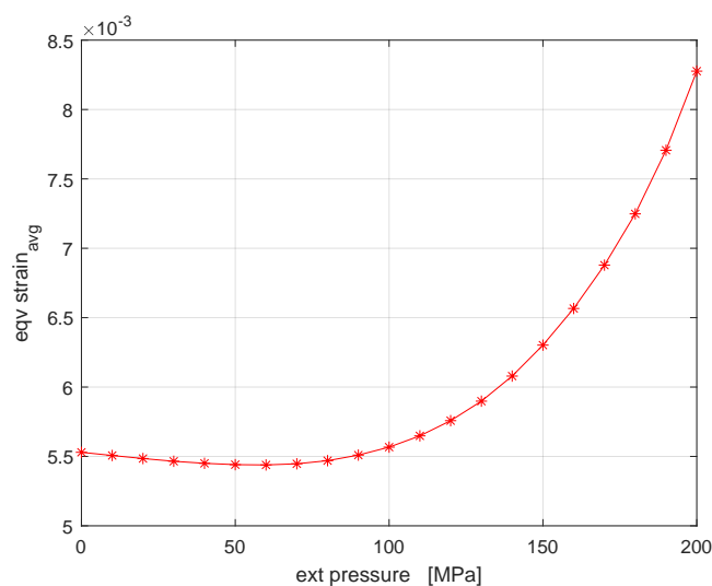
Figure 10: average equivalent strain in the strand's cross section as a function of the external transverse pressure with the effect of residual stress
