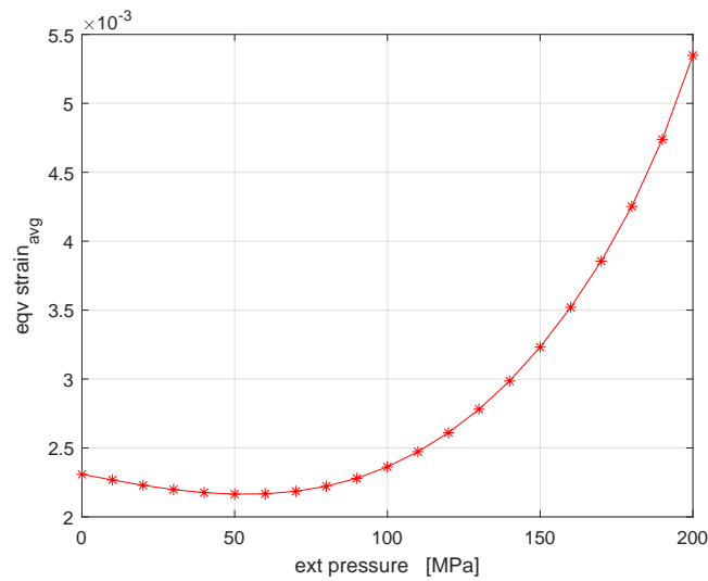
Figure 8: average equivalent strain in the strand’s cross section as a function of the external transverse pressure without the effect of residual stress
