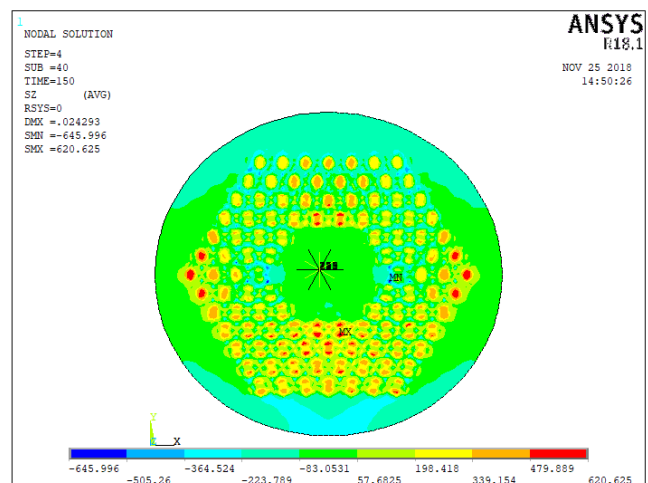
Figure 22: tensile test - \sigma_{eqv} , \sigma_{xx} , \sigma_{yy} , \sigma_{zz} at 100% load (external pressure = 200Mpa) and 4.2K with residual stress
