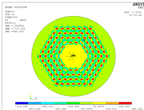
Figure 19: tensile test - \sigma_{eqv} , \sigma_{rr} , \sigma_{\theta\theta} , \sigma_{zz} at 100% load and 4.2K with residual stress
