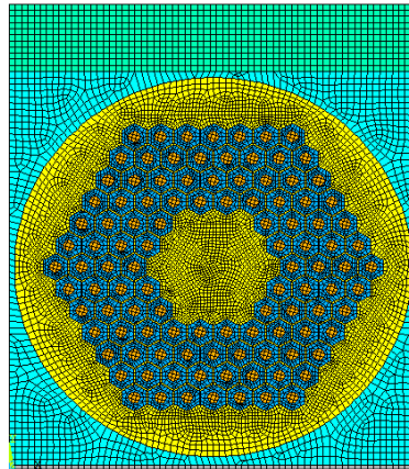
Figure 6: Ansys model used for transverse pressure test simulation
