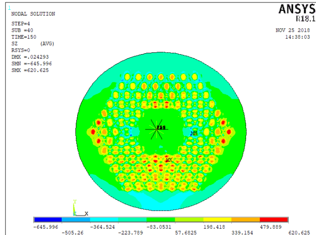
Figure 21: tensile test - \sigma_{eqv} , \sigma_{xx} , \sigma_{yy} , \sigma_{zz} at 0% load and 4.2K with residual stress
