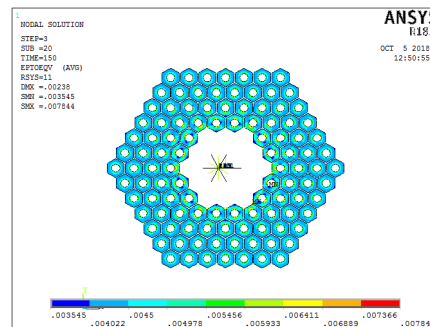
Figure 20: tensile test - equivalent strain in Nb 3 Sn at 0% and 100% load and 4.2K with residual stress
