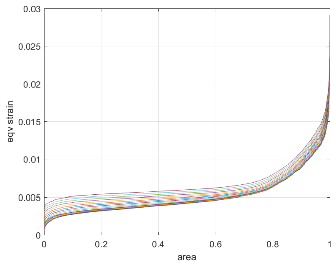
Figure 4: equivalent strain (function of area) in the strand cross section with increasing values of applied axial strain with the effect of residual stress
