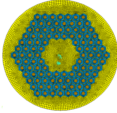
Figure 1: Ansys model used for tensile test simulation
