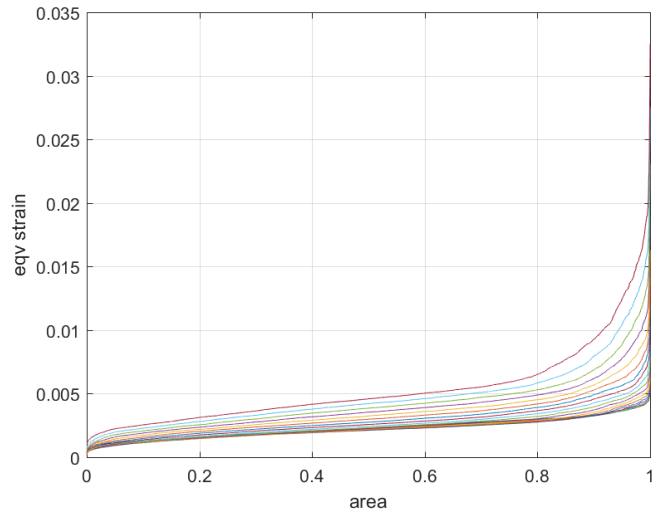
Figure 7: equivalent strain (function of area) in the strand’s cross section with increasing values of external transverse pressure without the effect of residual stress
