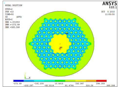
Figure 15: tensile test - \sigma_{eqv} , \sigma_{rr} , \sigma_{\theta\theta} , \sigma_{zz} at 0% load and 4.2K without residual stress
