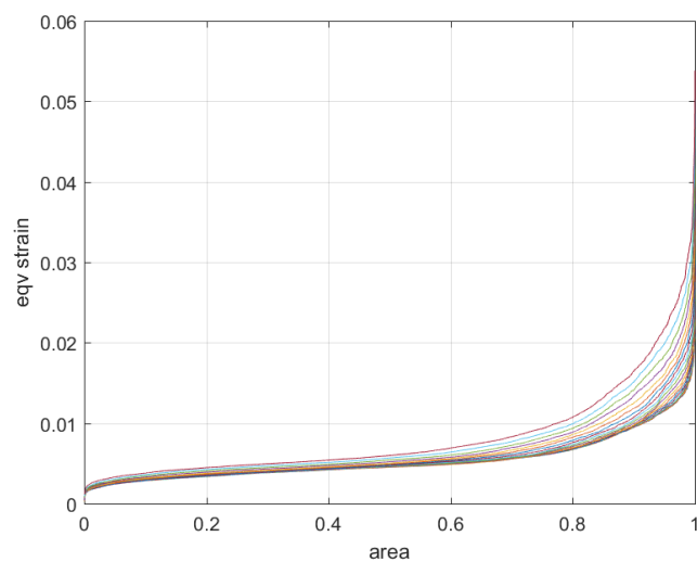
Figure 9: equivalent strain (function of area) in the strand's cross section with increasing values of external transverse pressure with the effect of residual stress
