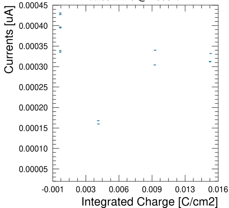
ALICE-2-0 @ 4000 V
