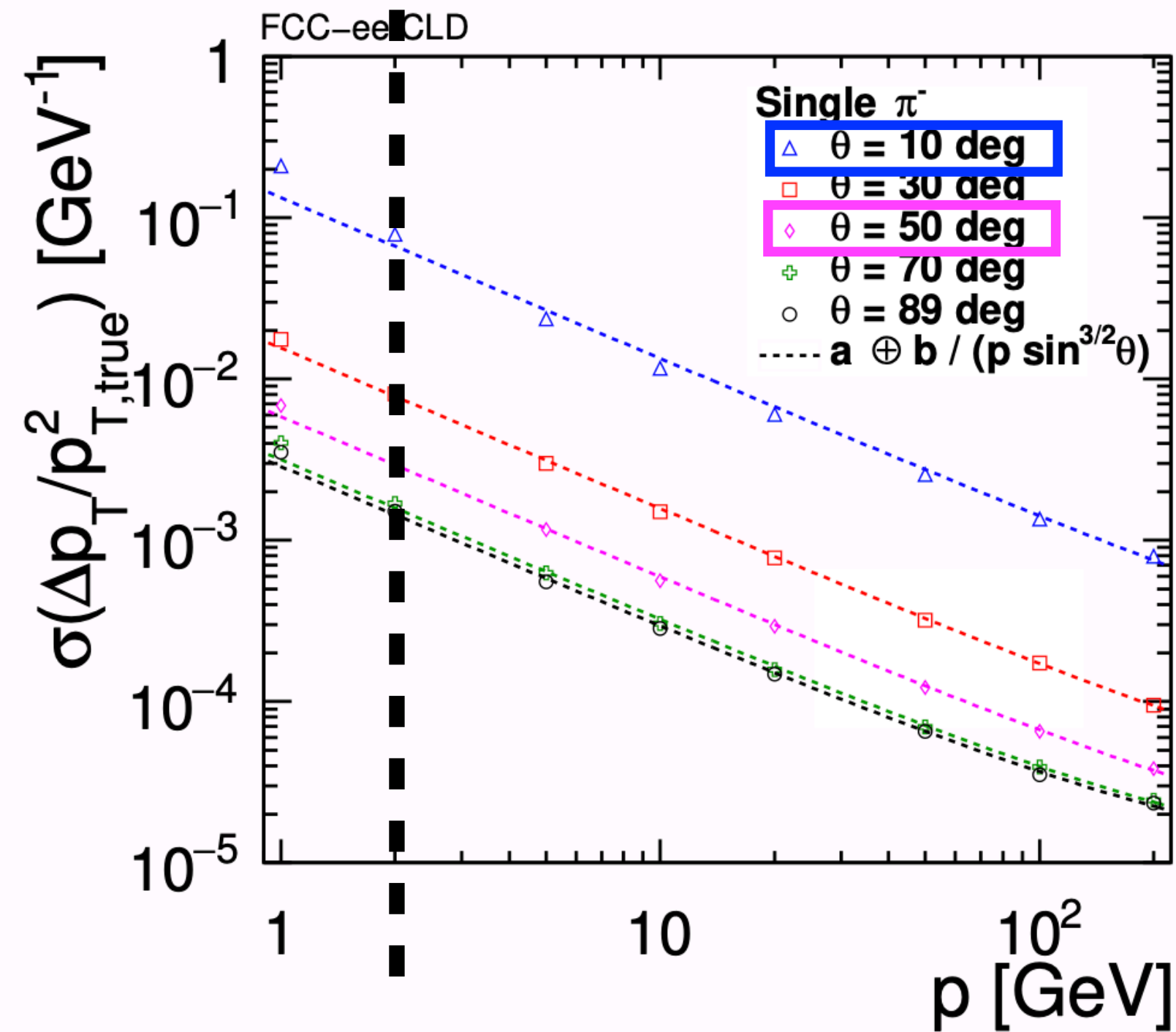
(b) pions
