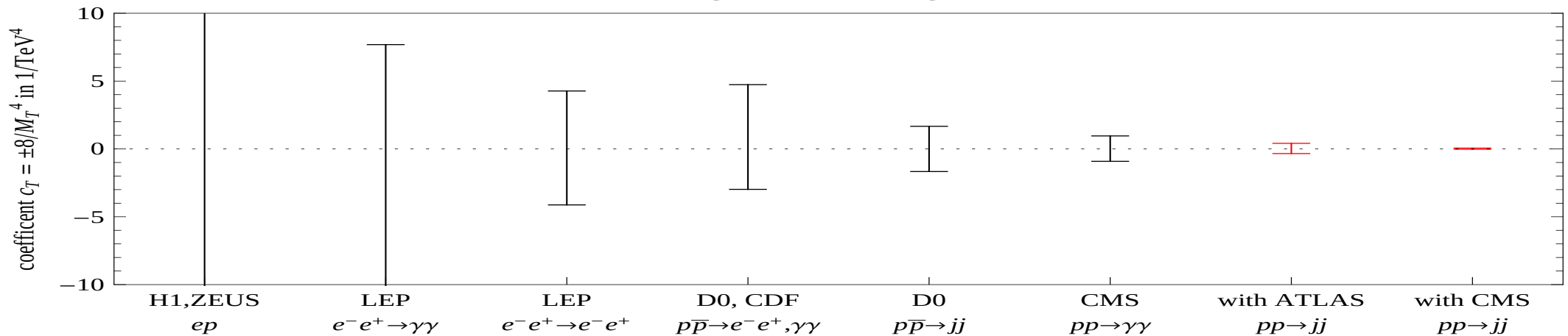
Bounds on graviton exchange at tree level
