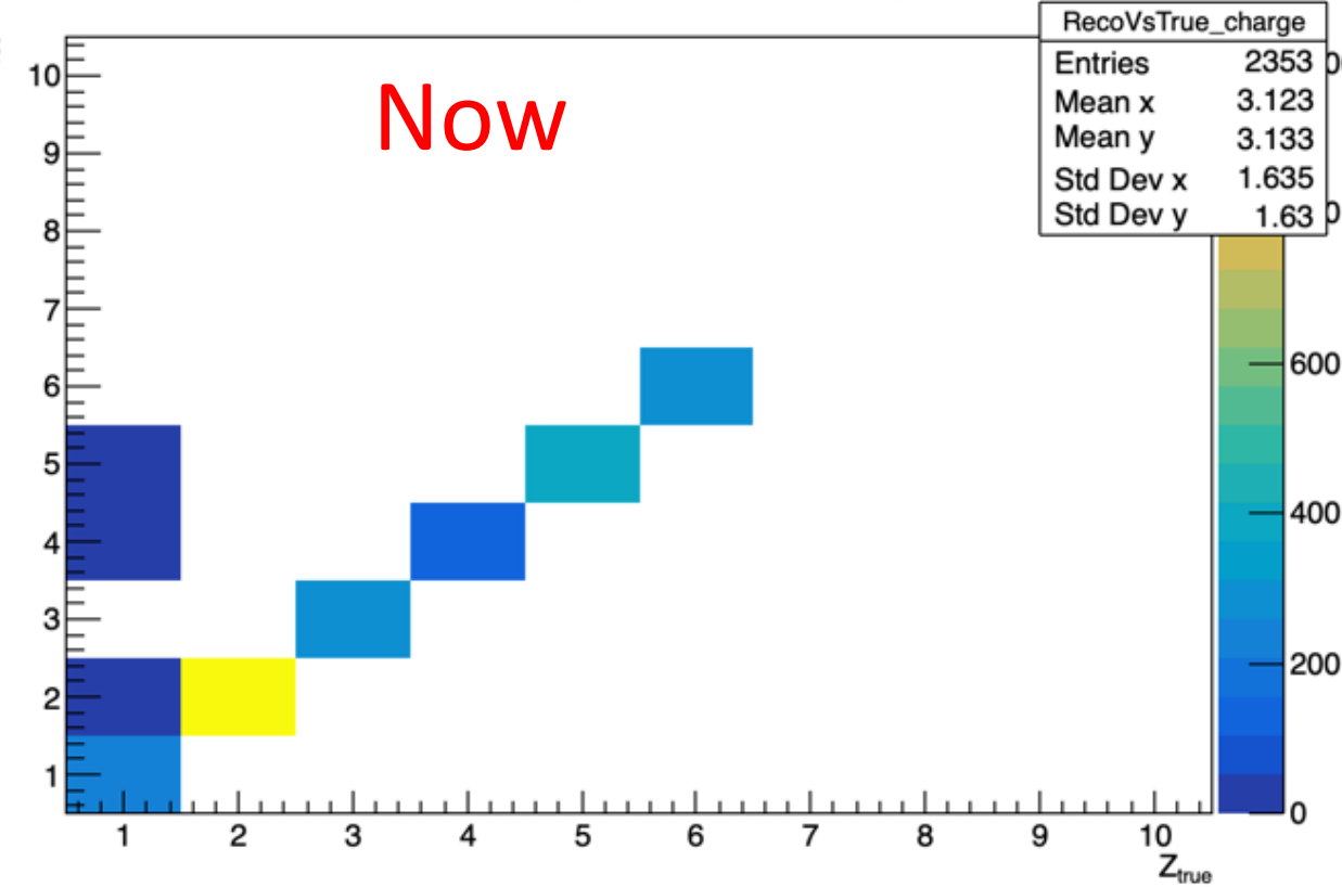
Reco Charge vs True Charge
