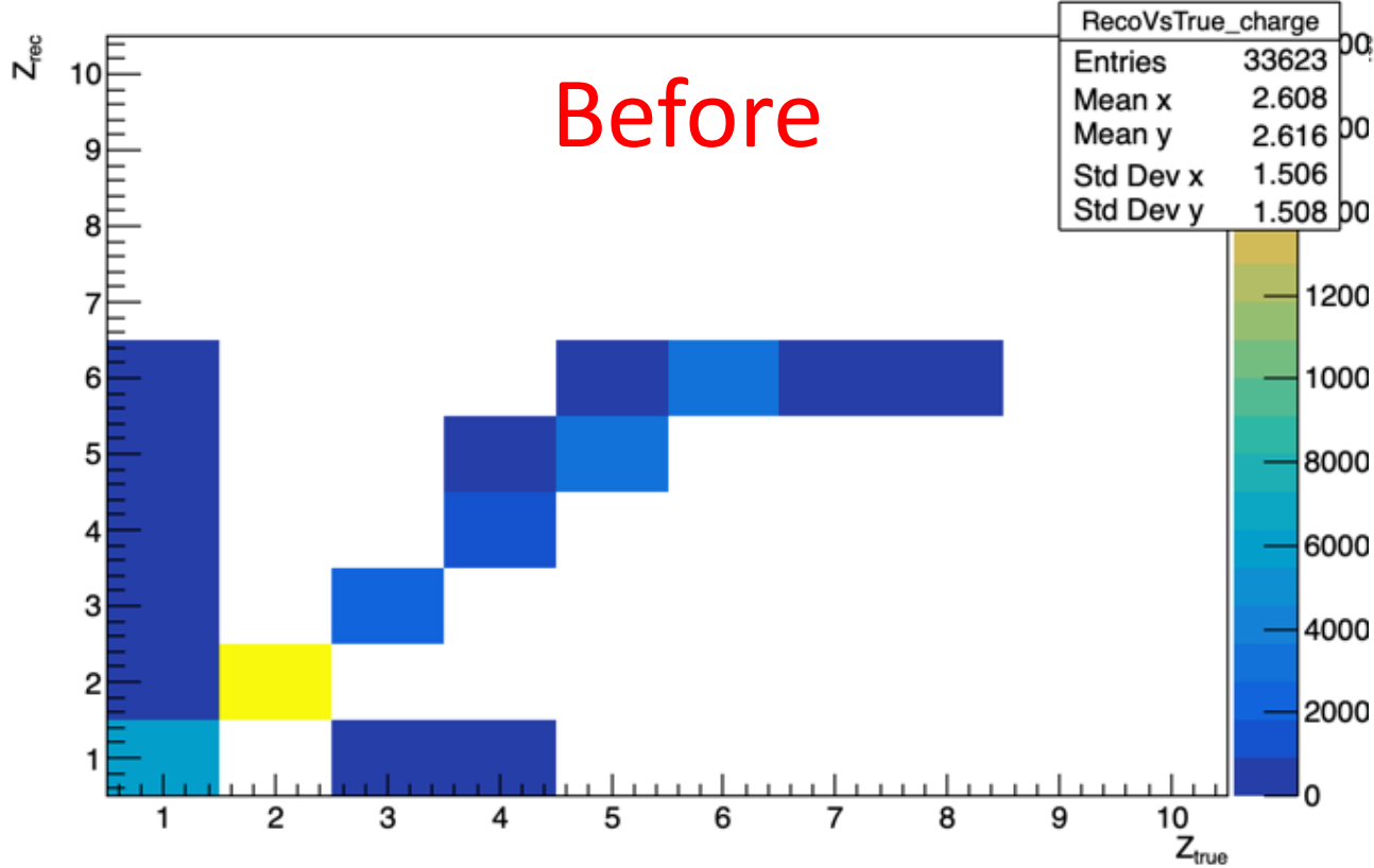
Reco Charge vs True Charge
